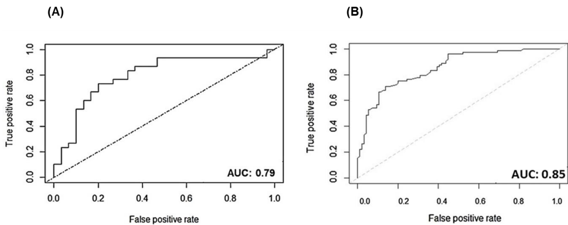
Figure 3. Receiver operating characteristics (ROC) curve for (A) performance of protein signatures in discovery cohort (MRM verification phase I, Total=60: 30 PsA; 30 RA) and (B) in an independent verification cohort (MRM verification phase II, Total=167: 95 PsA; 72 RA).
