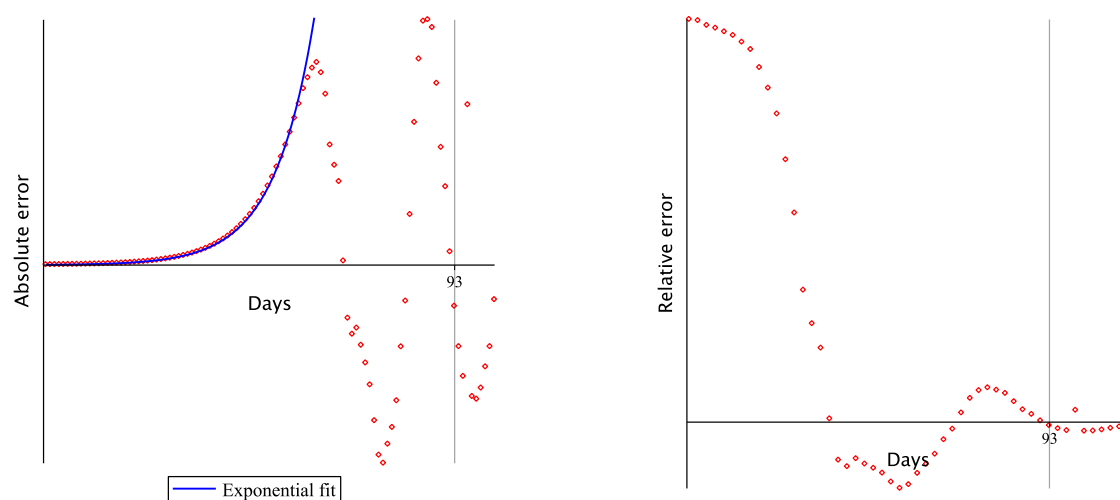
Fig. 2. The absolute and relative errors of forecasting the first wave. On the left, the blue line traces the exponential approximation of the discrepancy between actual and forecast data [6].
