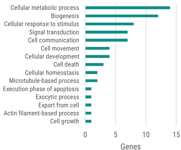
Figure 8: (A) Distributions of chromosomal locations for RF scored Genes. (B) Functional categories of genes defined by high-level Gene Ontology 15 terms.
