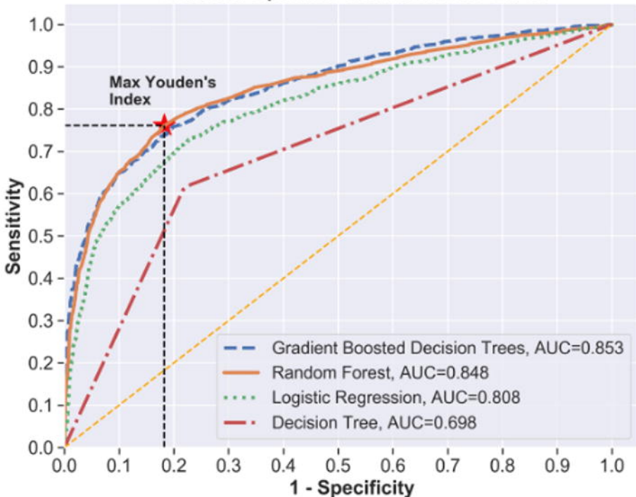
Receiver Operator Characteristic Curve
