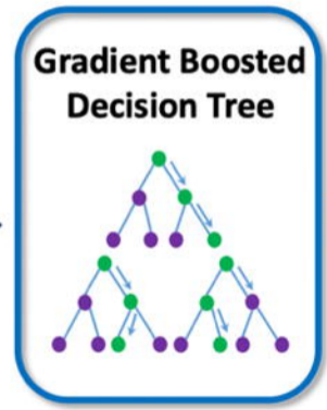
Classification
