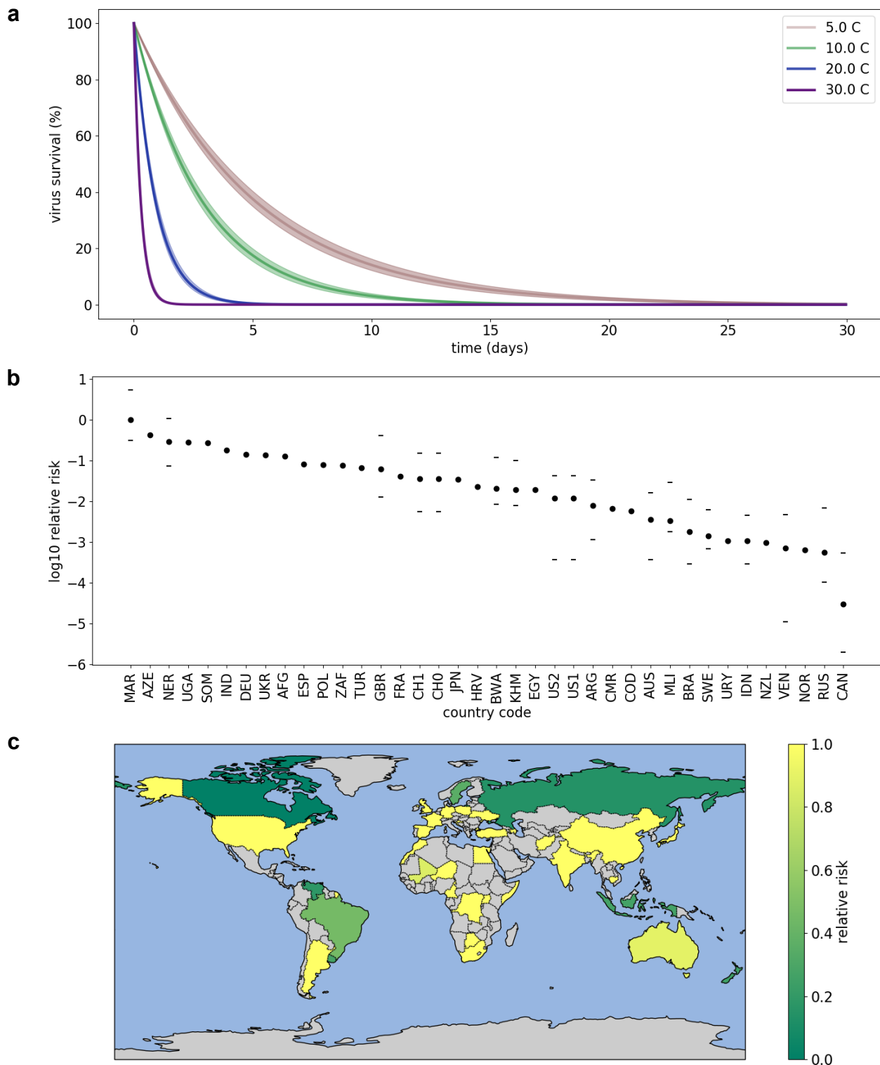
Figure 1 Virus survivability within water and relative risk posed by sewage spills into rivers for 39 countries; a) modelled temperature survivability. Shaded areas show the temperature dependent uncertainties; b) log 10 relative risk covering the range of 0.001 to 1.0; circles are median values, horizontal lines are 25 th and 75 th percentiles due to dilution factors from 13 and c) countries where relative risk has been calculated with relative risk as a linear scale; grey signifies a country not included.
