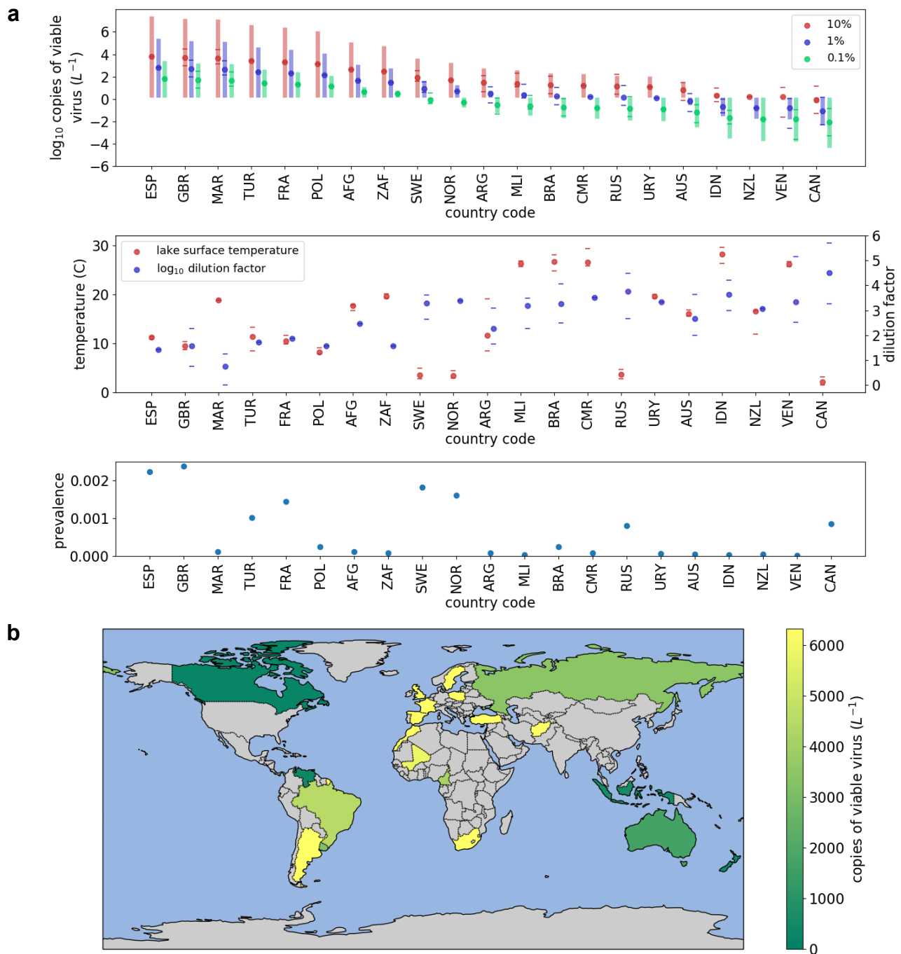
Figure 2 Estimate of absolute viable viral concentration within inland waters on the May 03 2020 for 21 countries assuming a sewage spill has occurred. a) absolute viable viral concentrations in \log_{10} copies. Circles are median, horizontal lines are 25 th and 75 th percentiles due to dilution factors from 13 ; shaded uncertainty bars are \pm 68\% copies L^{-1} . Results are shown for three possible ratios of viable virus to viral genome copies (10%, 1% and 0.1%) and b) countries where viable viral loads have been calculated. Grey signifies a country not included; viral concentrations are presented as a linear scale in copies of viable virus.
