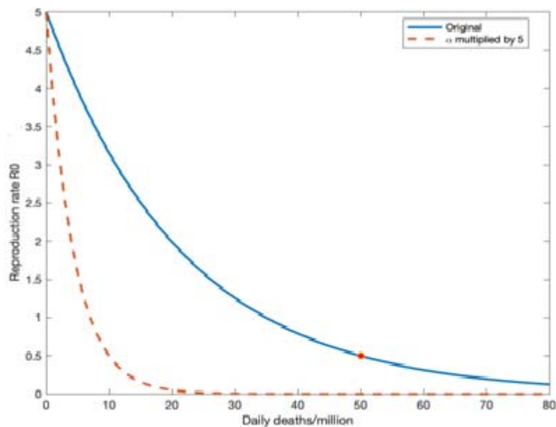
Figure 1: Reproductin rate, R_0 calibration [39]
