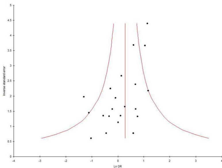
Figure 5 Funnel plot- precision by log odds ratio for allele contrast model (T vs. C) of total 24 studies of MTHFR gene C677T polymorphism.
