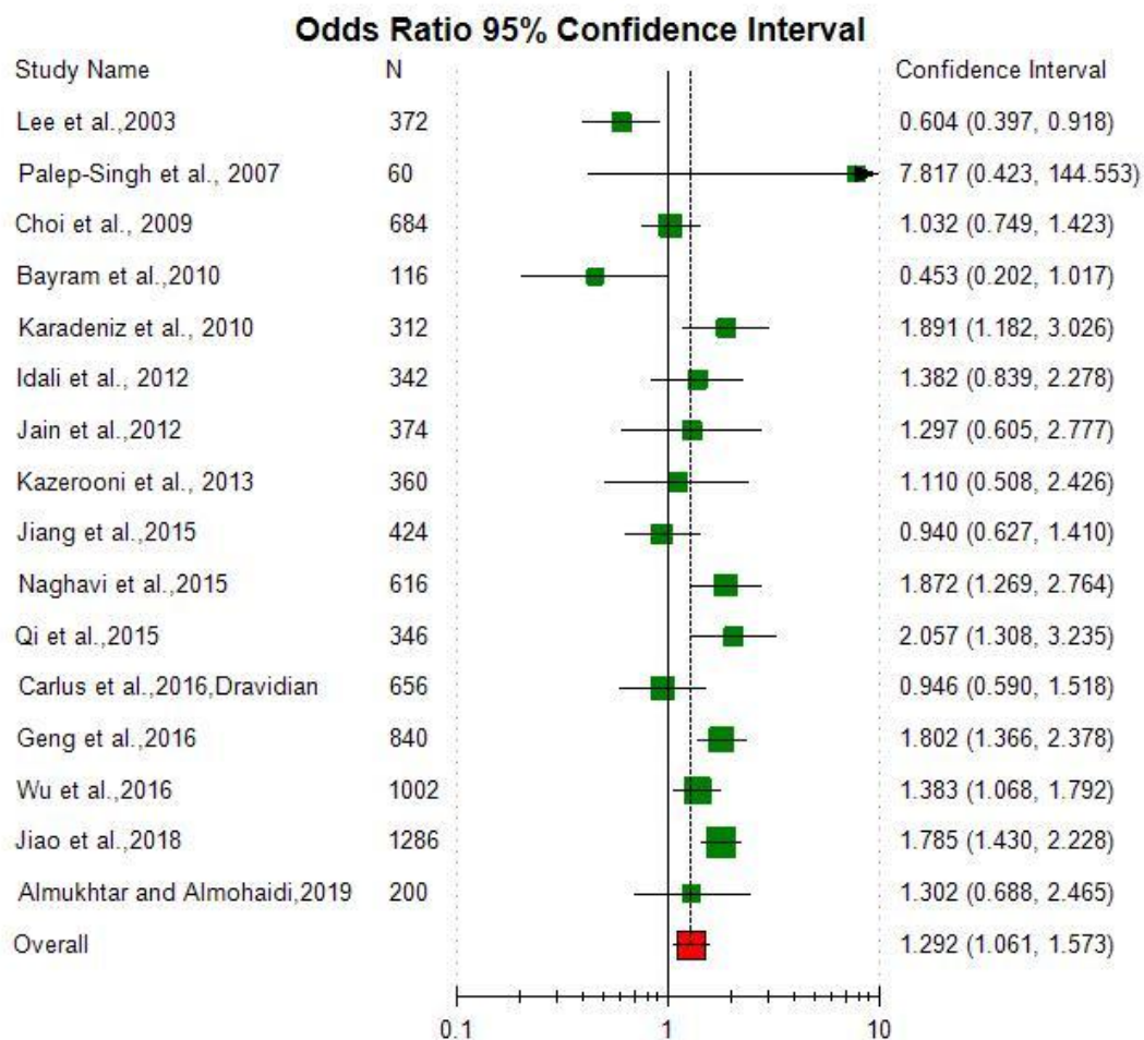
Figure 3. Random effect Forest plot of allele contrast model (T vs. C) of total 16 Asian studies of MTHFR gene C677T polymorphism.
