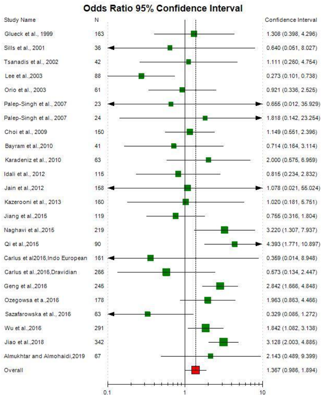
Figure 2. Random effect Forest plot of homozygote model (TT vs. CC) of total 24 studies of MTHFR gene C677T polymorphism.
