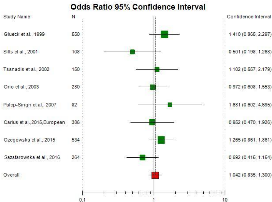
Figure 4. Random effect Forest plot of allele contrast model (A vs. G) of total 8 Caucasian studies of MTHFR gene C677T polymorphism.
