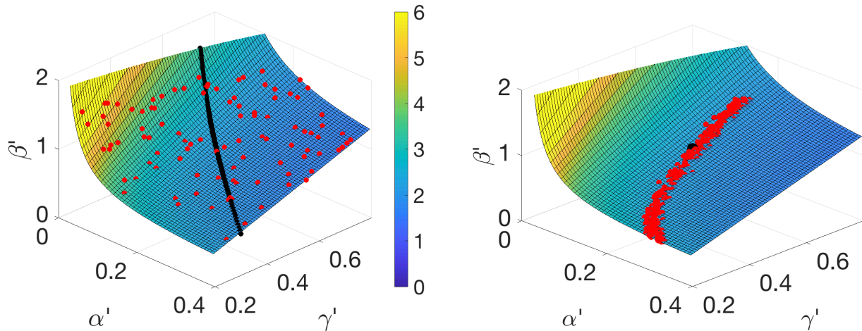
Figure 5: The unidentifiability surface defined by (10). (a) The red plotted points are the parameter values that minimized (landed in the smallest one percent of values) the loss function L(\beta, \alpha, \gamma) from the stochastic nonlinear SEIR model (1) trained on I(t) from the time interval [0, 50] . They are in remarkable agreement with the quadric surface (10) generated by the “non-generic” solutions. The black curve represents the parameter sets that generate the “generic” solutions from (6). The color represented on the surface corresponds to the computed R_0 = \beta'/\gamma' . (b) MCMC using I(t) on [0, 50] from the deterministic version of the nonlinear SEIR (1) to sample the posterior (red dots). They all lie on the surface (10). The true parameters are represented by the black dot.
