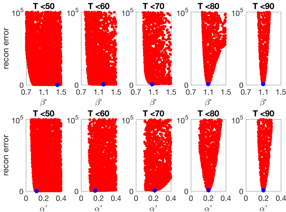
Figure 4: Estimation of parameters by minimization of data assimilation error on the time interval [0, T] for various T . Each red dot is the value of the sum of squares assimilation error for randomly chosen parameters (\beta', \alpha') , while the exact \gamma' = \gamma = 0.5 is assumed known. The blue dot represents the calculated minimum. For T significantly below 80, the loss function has no well-defined minimum, and the generating parameters (\beta = 1.1, \alpha = 0.2) are poorly estimated. For larger T , the minimum becomes more pronounced and the parameters can be well estimated.
