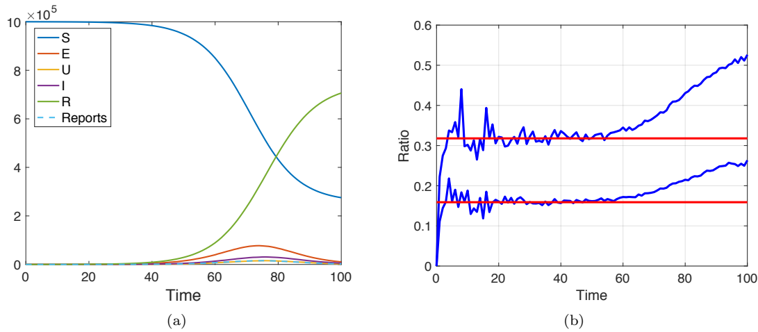
Figure 8: (a) Solution of the stochastic SEUIR equations (13) with initial conditions S = 10^6, E = 10^2, U = 0, I = 0, R = 0 . The parameter settings are \beta = 0.9, z = 0.3, w = 0.2, d = 0.5 . (b) Ratios U(t)/E(t) and I(t)/E(t) (blue traces) compared with b = 0.16 and c = 0.32 calculated from (15), shown in red.
