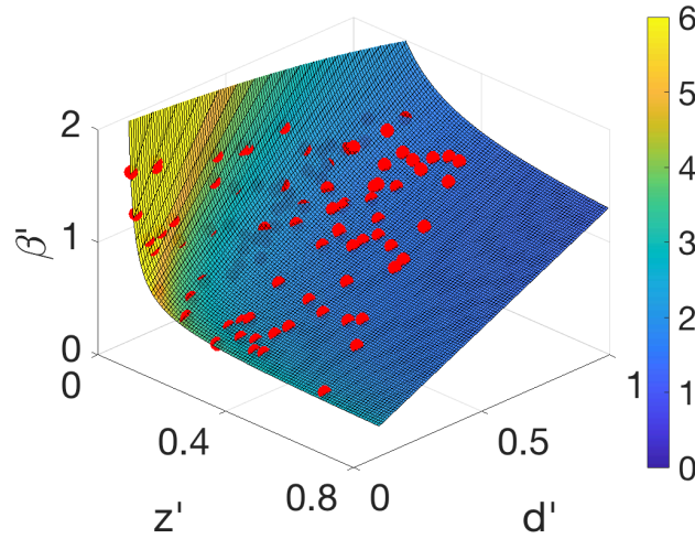
Figure 9: The unidentifiability surface defined by (17). The red plotted points are the parameter values that minimized (landed in the smallest one percent of values) the loss function L(\beta', z', d') from the nonlinear SEUIR model (13), where w' = w = 0.2 was assumed known. The parameters generating the input I(t) were (\beta, z, w, d) = (0.9, 0.3, 0.2, 0.5) . The input I(t) was used from the pre-peak time interval [0, 50] . The surface is colored corresponding to R_0 .
