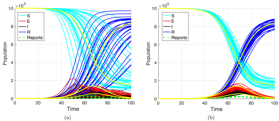
Figure 7: Trajectories of 30 systems with alternative parameter values. (a) Parameter values p'' = (\beta'', \alpha'', \gamma'') are chosen by perturbing randomly with 10% Gaussian noise from a fixed p' = (\beta', \alpha', \gamma') = (0.852, 0.25, 0.4) . The original trajectory with parameter values p = (\beta, \alpha, \gamma) = (1.1, 0.2, 0.5) is traced in yellow. (b) Same as (a), but the p'' are chosen from the surface. Specifically, the p'' are formed by perturbing (\alpha'', \gamma'') by 10% and calculating the corresponding \beta'' lying on the surface.
