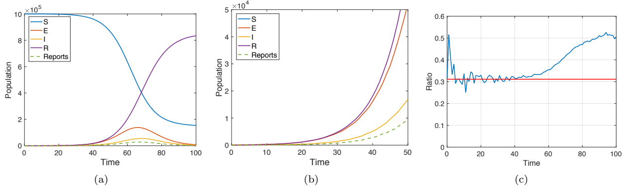
Figure 3: Plot of SEIR populations with parameters \beta = 1.1, \alpha = 0.2, \gamma = 0.5 . The new cases \Delta I are denoted by the dashed curve (Reports in the legend). (a) Full plot on [0, 100] . (b) Magnification of (a), restricted to the time interval [0, 50] . (c) The blue curve is a plot of the ratio I(t)/E(t) . Here I \approx cE for the first 50 days, where c = 0.31 , as calculated from (8).
