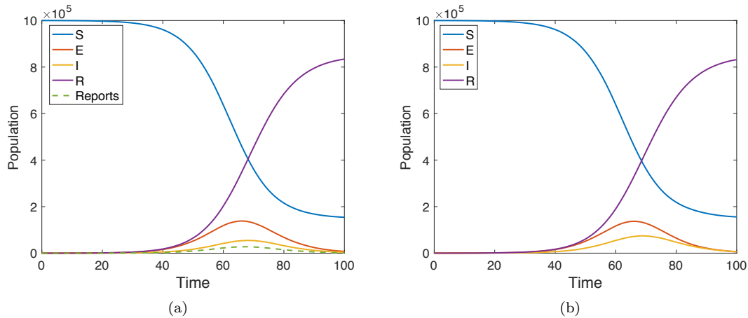
Figure 1: (a) Solution of the SEIR equations (1) with initial conditions S = 10^6, E = 10^2, I = 0, R = 0 . The parameter settings are \beta = 1.1, \alpha = 0.2, \gamma = 0.5 . (b) Result of data assimilation using exact parameters of model with initial conditions S = 10^6, E = 0, I = 0, R = 0 , and the reports \Delta I as inputs.
