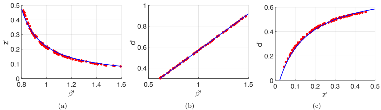
Figure 10: Continuous families of best parameter sets that share the same I(t) . The dots denote the one percent of pairs (chosen from 10000 random pairs) with the smallest sum of squares error L from data assimilation over the interval [0, 50] . The solid curve is (17) with \Delta w = 0 and (a) \Delta d = 0 , (b) \Delta z = 0 , (c) \Delta \beta = 0 .
