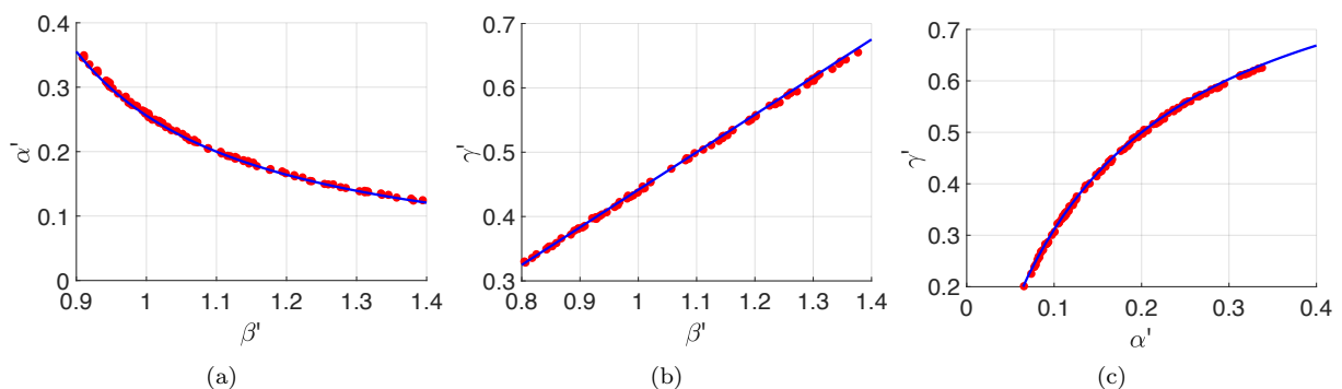
Figure 6: Continua of best parameter sets from the same I(t) . (a) The dots denote the one percent of (\beta', \alpha') pairs (chosen from 10000 random pairs) with the smallest sum of squares error from data assimilation over the interval [0, 50] . The blue curve is given by equation (10) with \beta', \alpha', c as in Figure 3, and setting \gamma = \gamma' = 0.5 . (b) The dots are the (\beta', \gamma') pairs with smallest assimilation error for fixed \alpha = \alpha' = 0.35 . Equation (10), plotted as the blue dashed curve, is the line \gamma' = \gamma + \alpha(\beta' - \beta)/(c\beta) . (c) The dots are the (\alpha', \gamma') pairs with smallest assimilation error for fixed \beta = \beta' = 0.7 . The red dashed curve is \gamma' = \gamma + (\alpha'\beta c)/(\alpha' + \beta c - \alpha) - \alpha/c from (10) setting \beta = \beta' = 0.7 .
