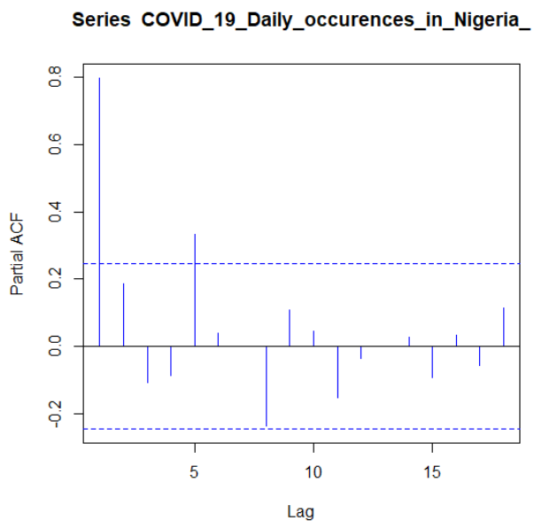
Fig 5: PACF Plot
