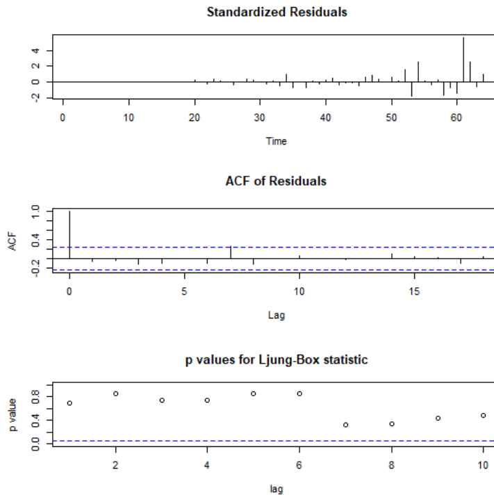
Fig 6: Diagnostic plot
