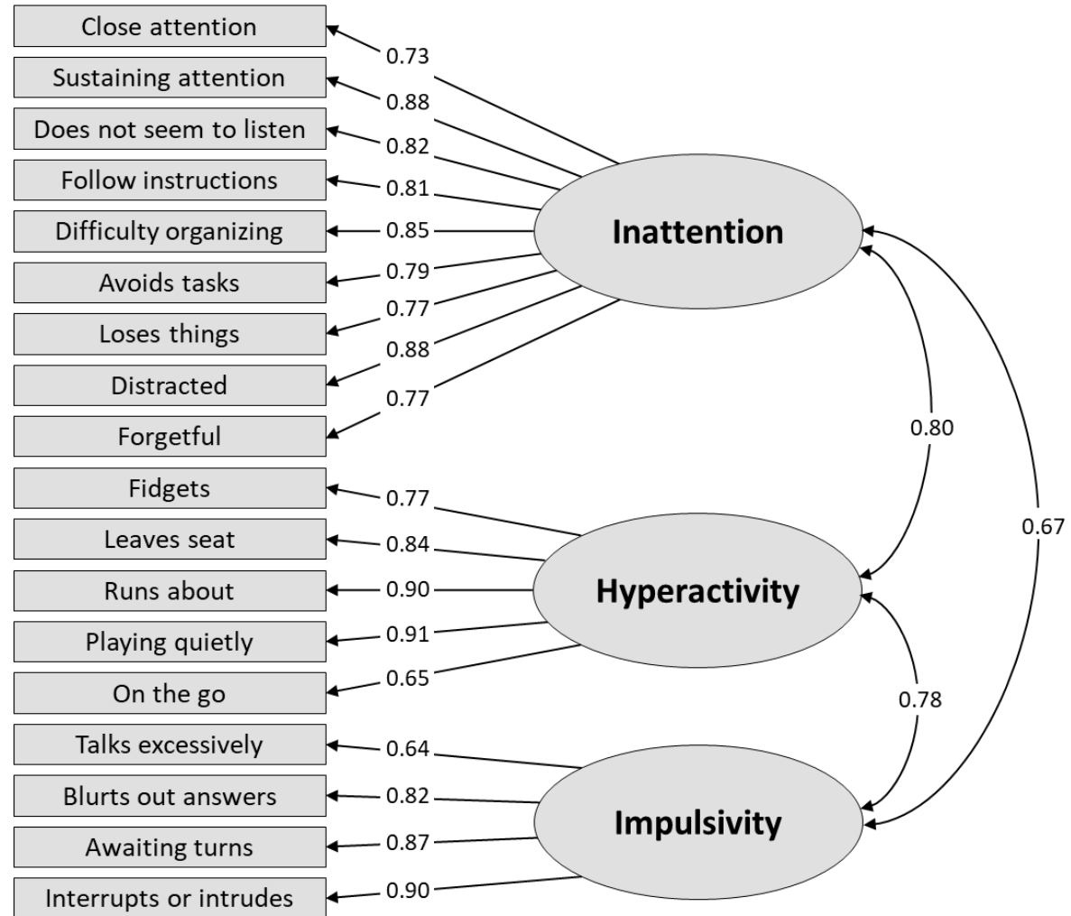
Figure S4 Correlated three-factor model with “talk excessively” as part of the Impulsivity factor in the general population sample (N=2044)
