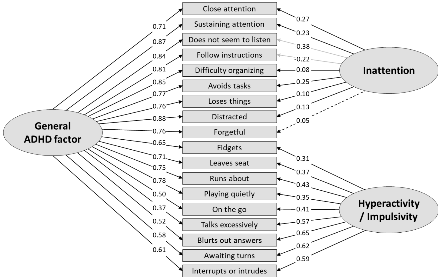
Figure S5 Bifactor model with two specific factors in the general population sample (N=2044)
