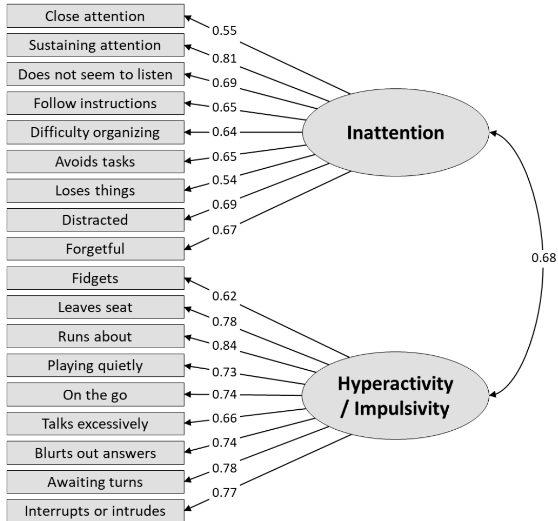
Figure S9 Correlated two-factor model in the ADHD sample (N=147)
