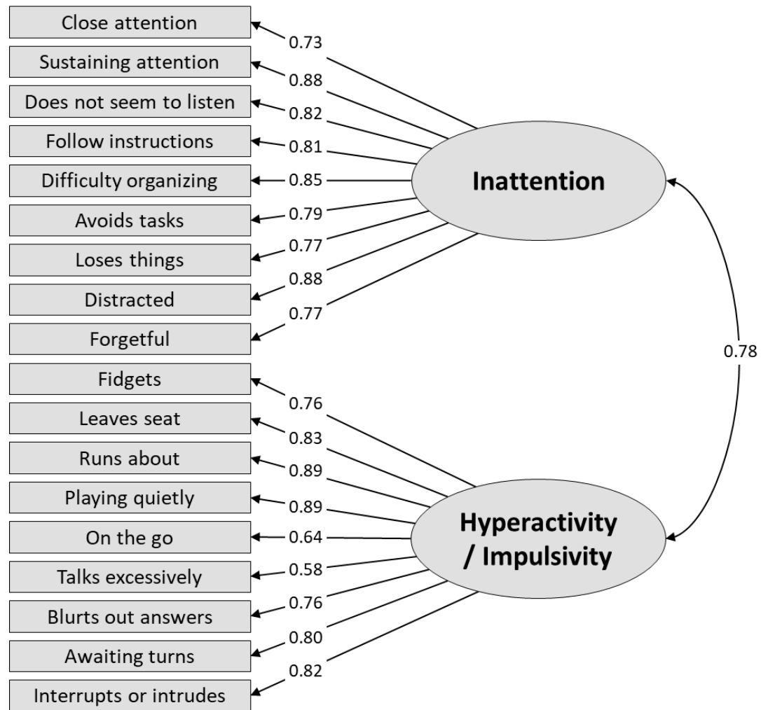
Figure S2 Correlated two-factor model in the general population sample (N=2044)
