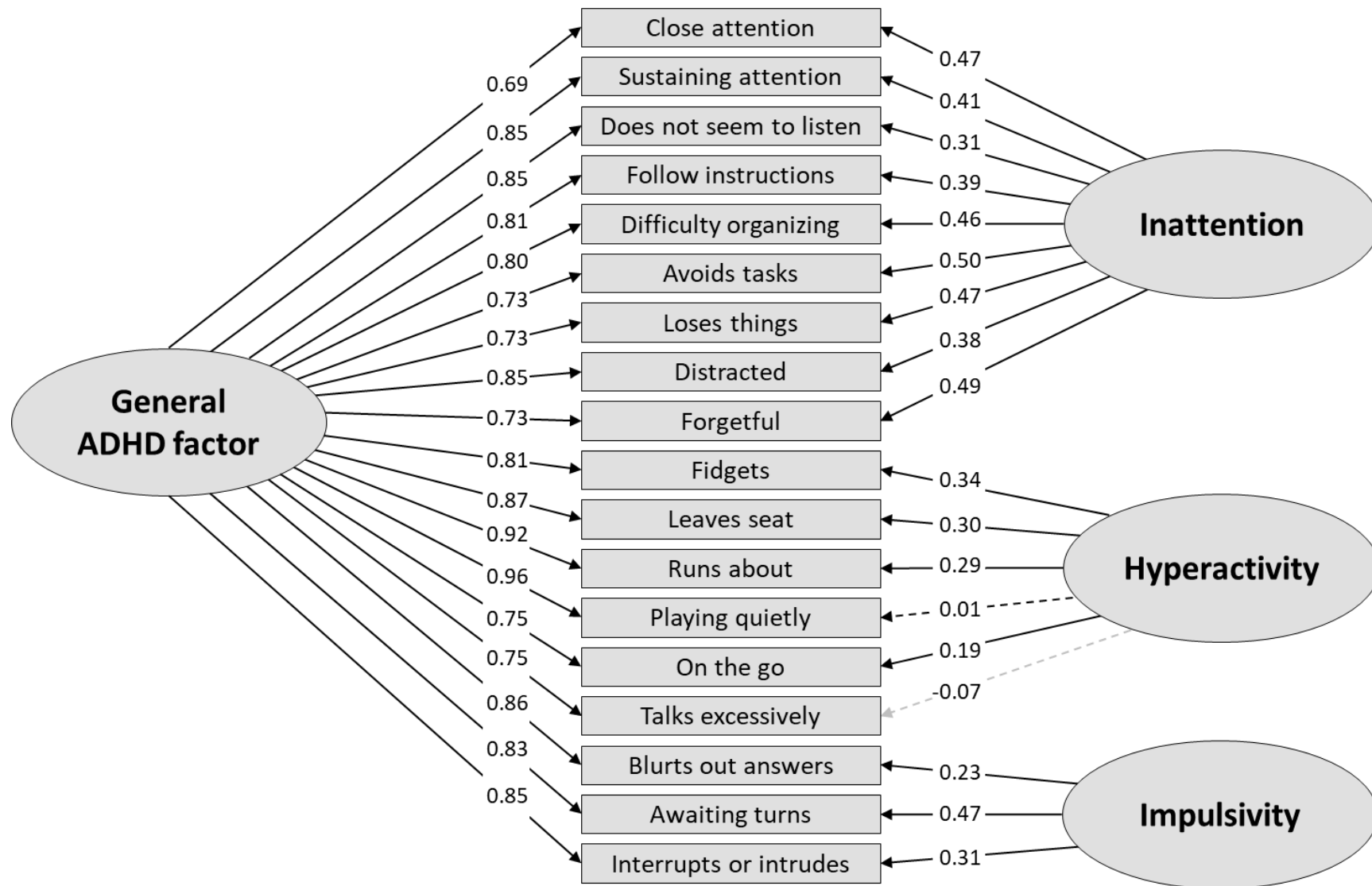
Figure S6 Bifactor model with three specific factors with “talk excessively” as part of the specific Hyperactivity factor in the general population sample (N=2044)
