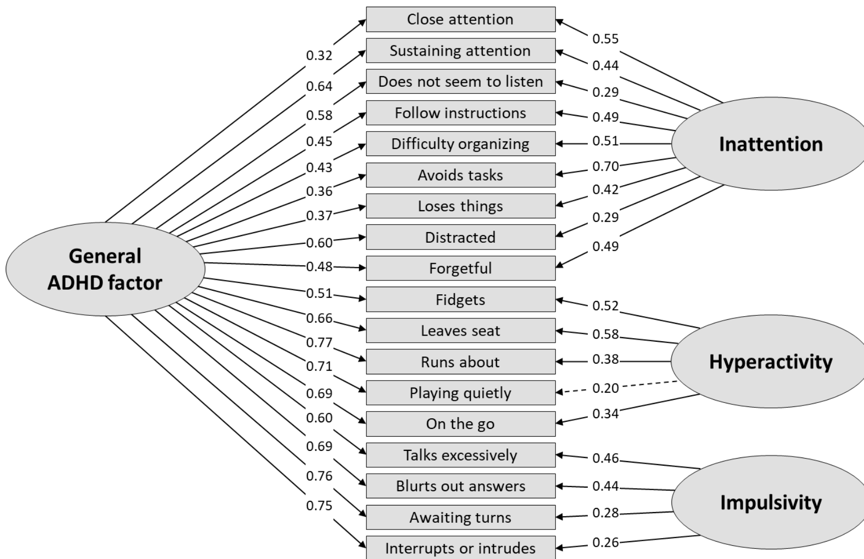
Figure S14 Bifactor model with three specific factors with “talk excessively” as part of the specific Impulsivity factor in the ADHD sample (N=147)
