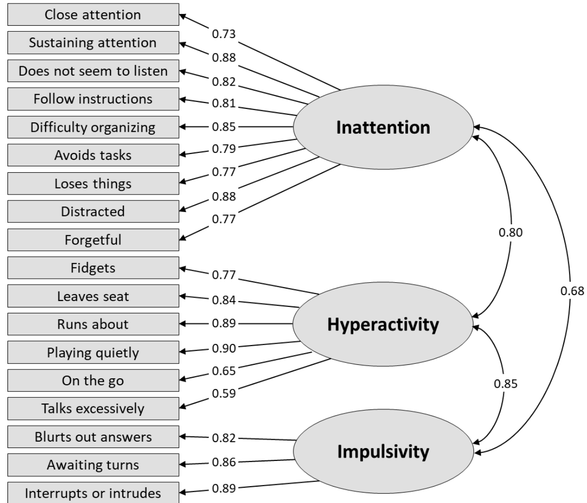
Figure S3 Correlated three-factor model with “talk excessively” as part of the Hyperactivity factor in the general population sample (N=2044)
