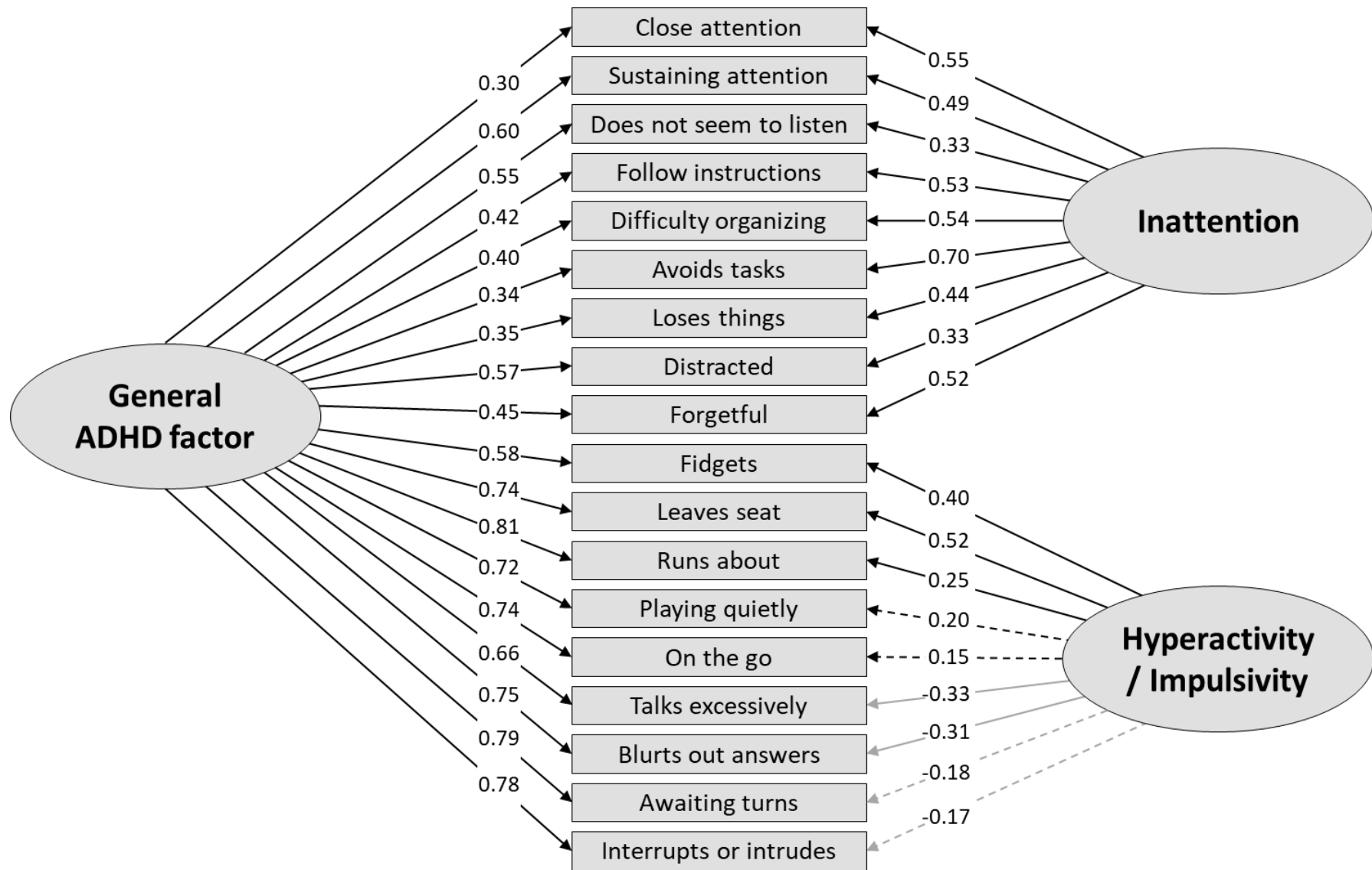
Figure S12 Bifactor model with two specific factors in the ADHD sample (N=147)
