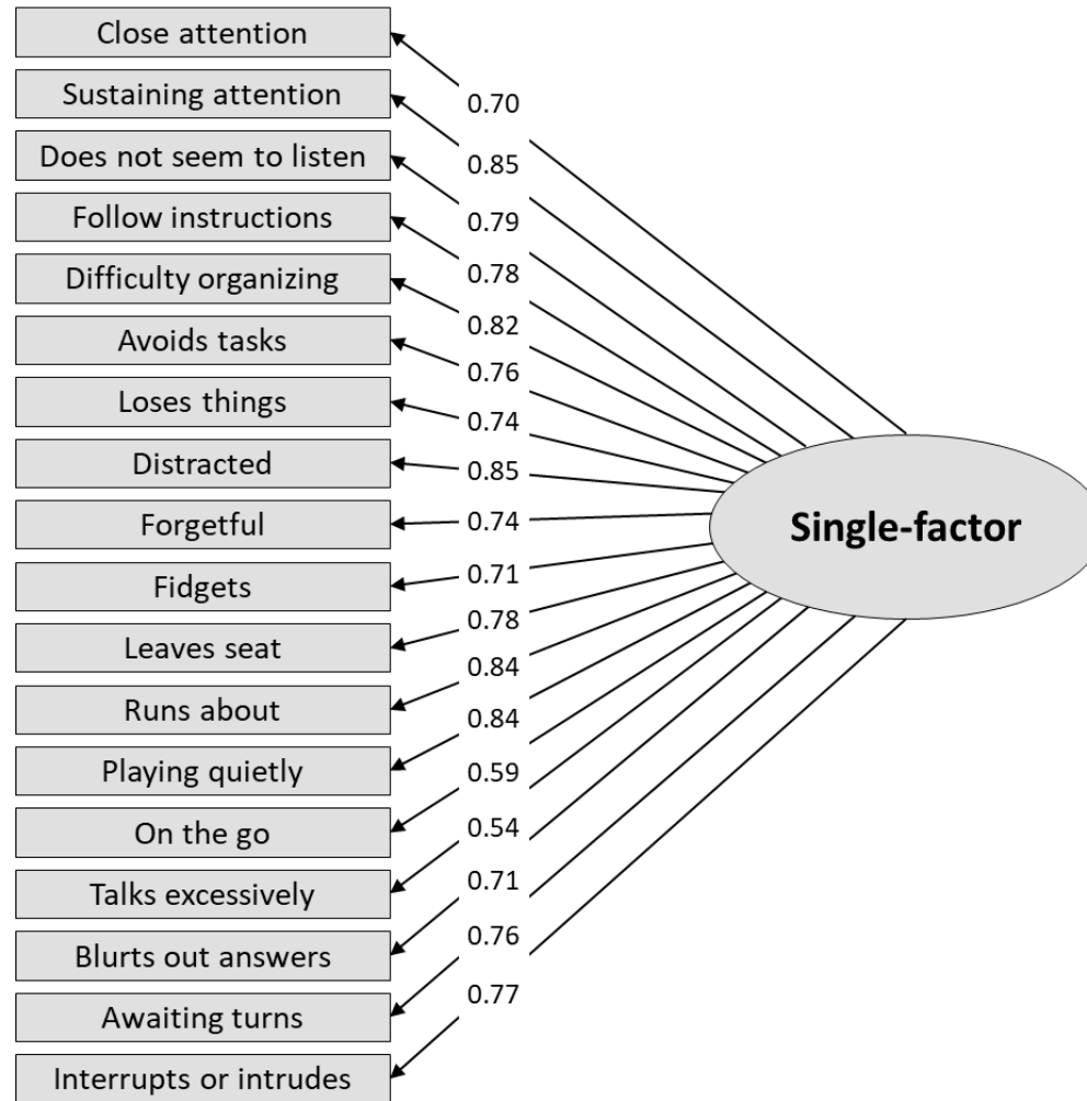
Figure S1 Single-factor model in the general population sample (N=2044)
