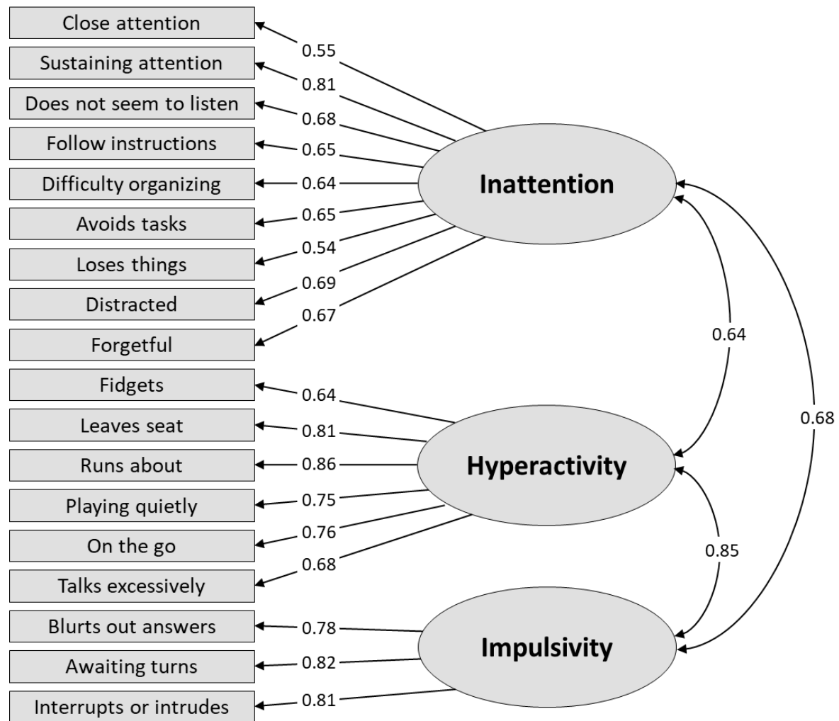
Figure S10 Correlated three-factor model with “talk excessively” as part of the Hyperactivity factor in the ADHD sample (N=147)
