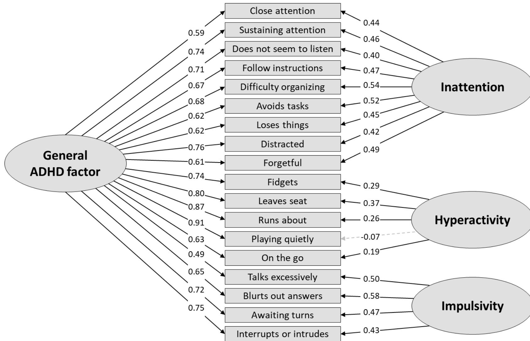
Figure S7 Bifactor model with three specific factors with “talk excessively” as part of the specific Impulsivity factor in the general population sample (N=2044)
