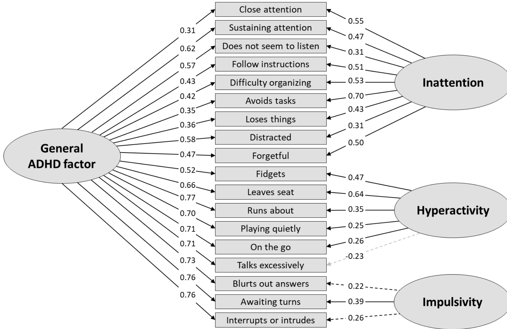
Figure S13 Bifactor model with three specific factors with “talk excessively” as part of the specific Hyperactivity factor in the ADHD sample (N=147)
