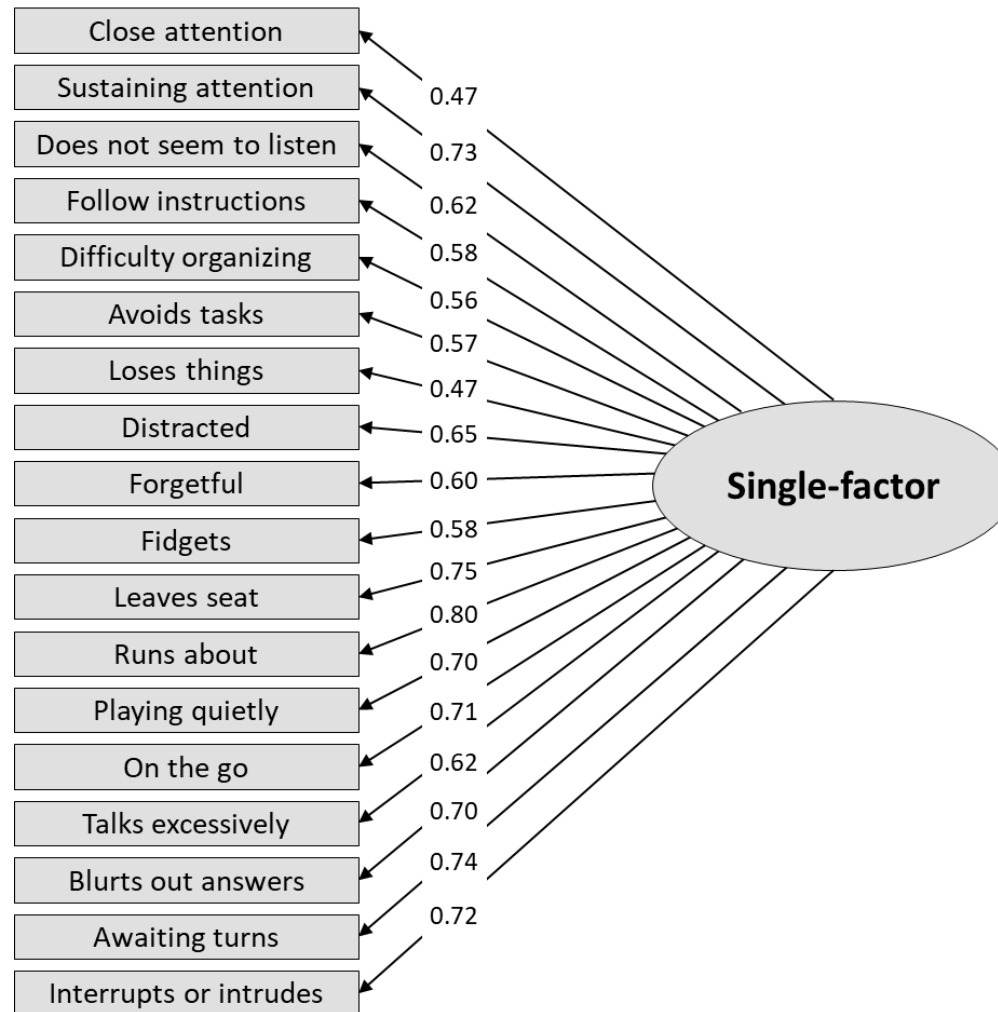
Figure S8 Single-factor model in the ADHD sample (N=147)
