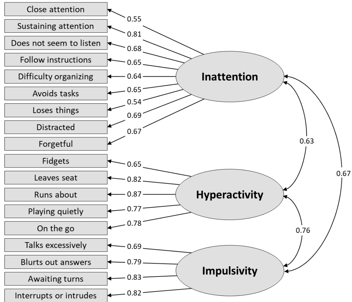
Figure S11 Correlated three-factor model with “talk excessively” as part of the Impulsivity factor in the ADHD sample (N=147)
