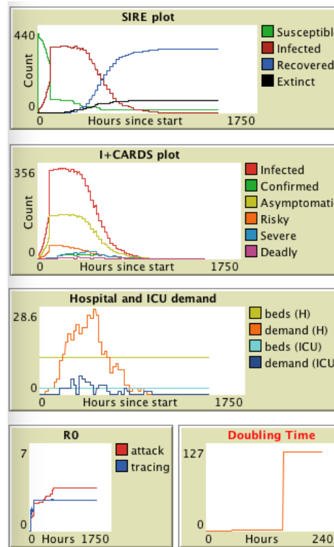
Figure 14. Plots of a single run of TL simulation.
