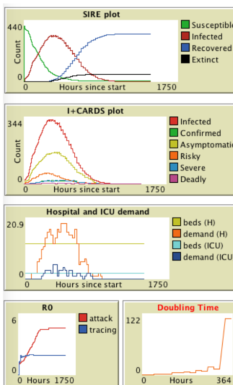
Figure 8. Plots of a single run of SD simulation.
