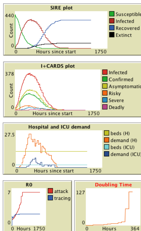
Figure 10. Plots of a single run of CI simulation.
