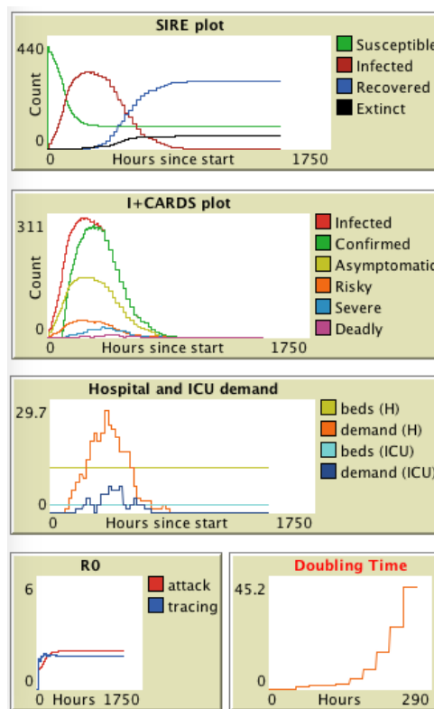
Figure 12. Plots of a single run of ST simulation.
