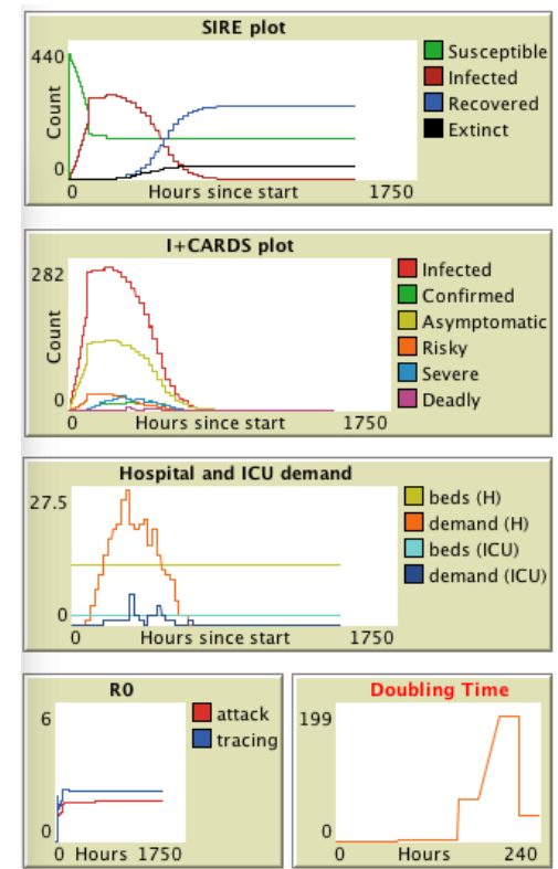
Figure 15. Plots of a single run of TL+ZE simulation.
