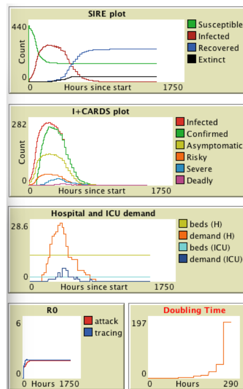
Figure 13. Plots of a single run of ST+ZE simulation.
