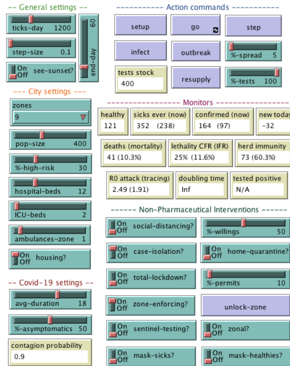
Figure 4. Control panel of the simulation tool.
