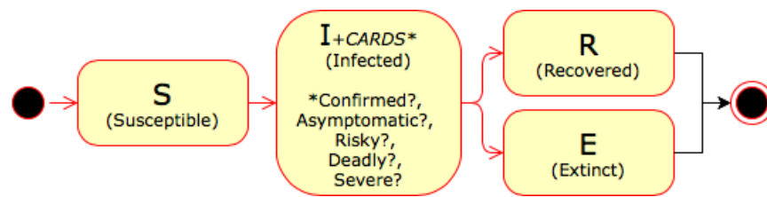
Figure 1. Schematic of the SIRE+CARDS state model.
