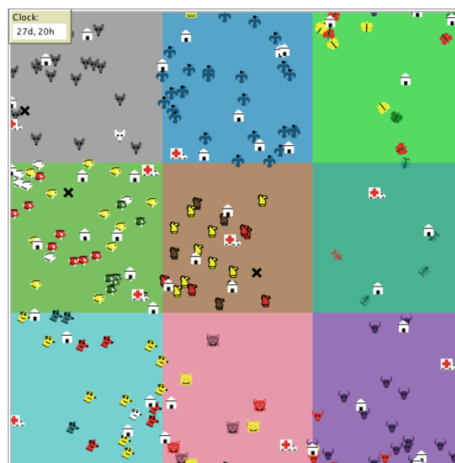
Figure 3. View area of the simulation tool. Agents are identified by a different shape and colour per zone; additionally, the epidemic state of agents is indicated by red (symptomatic), yellow (asymptomatic) or white (recovered, immune); deaths are shown by black cross marks (x). Besides, households and sentinels (ambulances) can also be seen.
