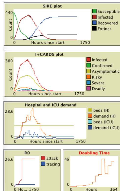
Figure 7. Plots of a single run of ZE simulation.
