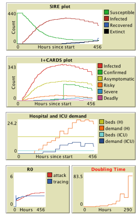
Figure 5. Plot area of the simulation tool.
