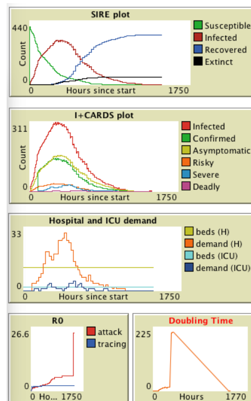
Figure 11. Plots of a single run of CI+ZE simulation.
