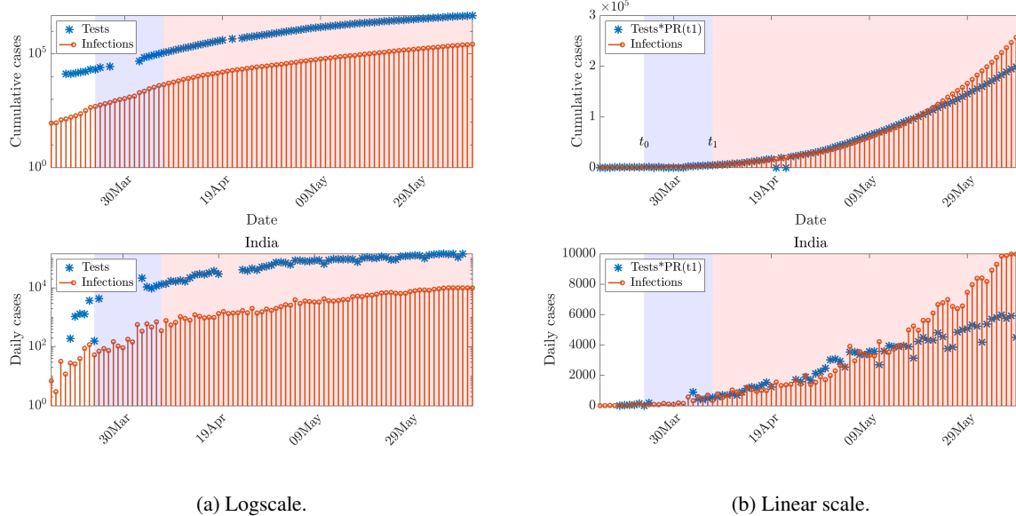
Figure 4: Comparison of Covid-19 growth in India with diagnostic test data. The shaded region show the period from implementation of lockdown ( t_0 ) to t_1 = t_0 + 14 .
