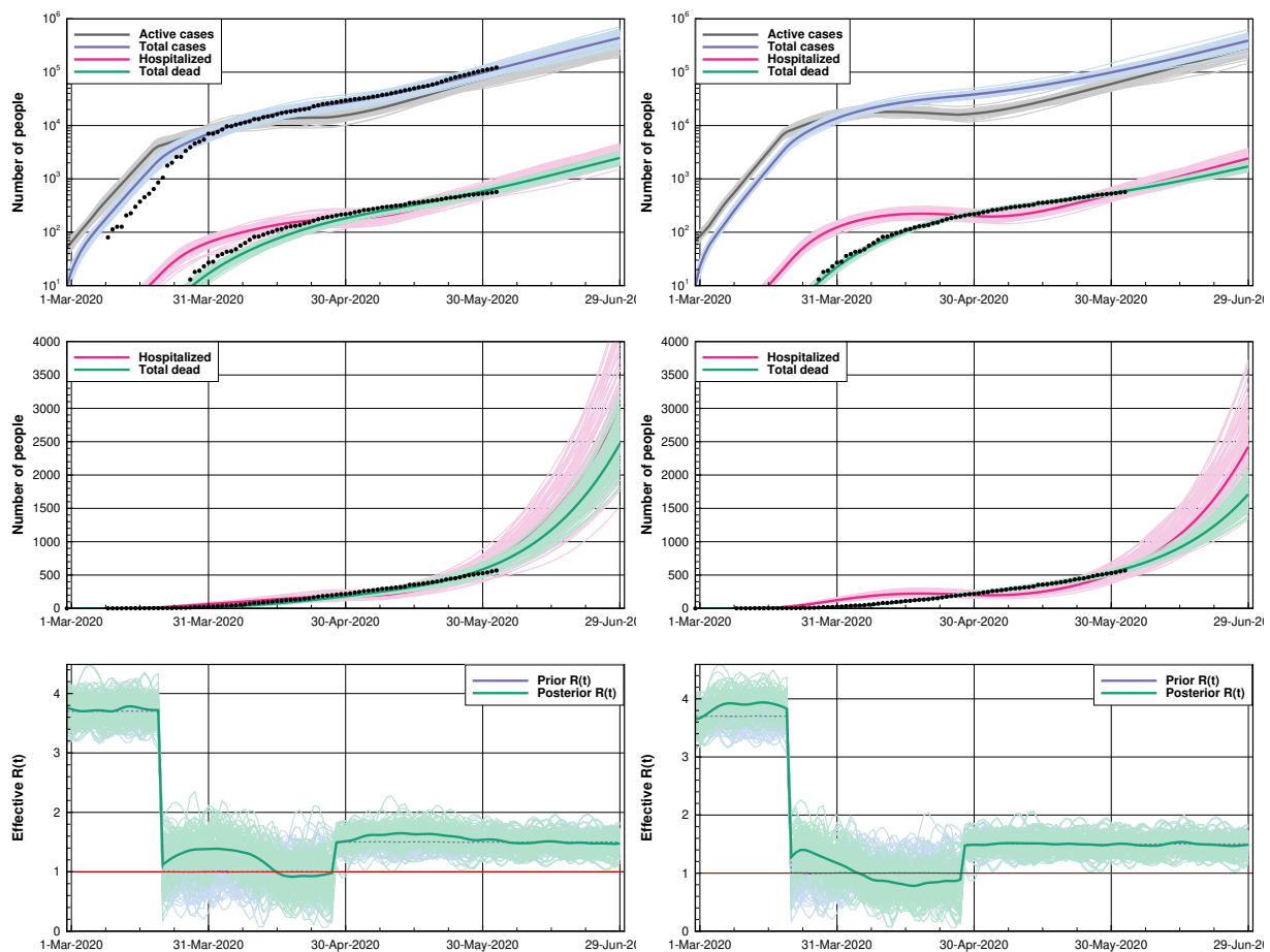
FIGURE 16. Argentina: The dots are the observations. In Case 1 (left plots) both the accumulated deaths and the estimated number of cases were conditioned on, while in Case 2 (right plots) we only conditioned on the total number of deaths.
