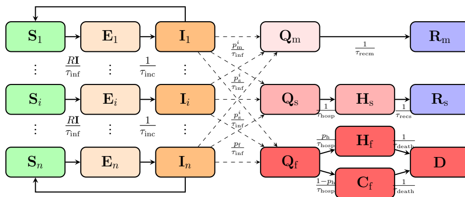
FIGURE 1. Flow diagram of the SEIR model
