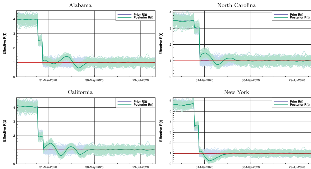
FIGURE 21. US Case 3: A gradual step down in R(t) with the first and intermediate values chosen so that the prior mean closely follows the data until the time for which R(t) is guessed to be one.
