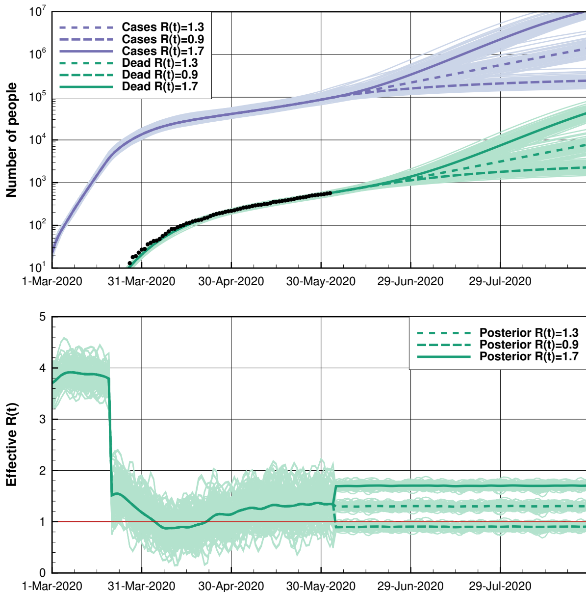
FIGURE 17. Argentina: Same as Figure 16 but for an experiment focused on a probabilistic prediction in which three scenarios, with different effective reproductive numbers imposed from June 1st, R(t) = 1.7, 1.3, and 0.9 .
