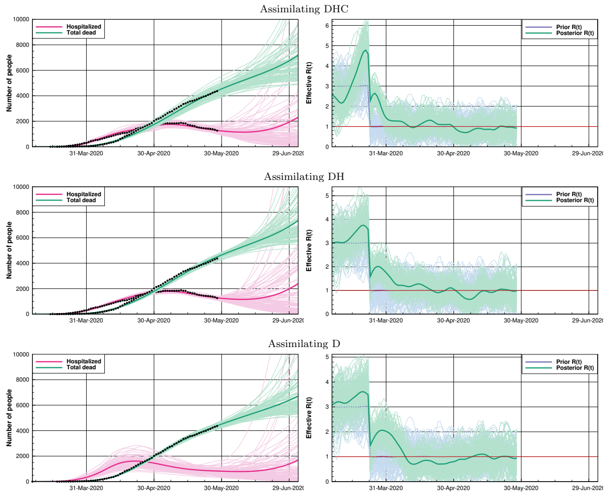
FIGURE 6. Quebec: From top to bottom, the plots show the results from the three assimilation experiments DHC, DH, and D. The left column presents the accumulated number of deaths and the number of hospitalizations, and the right column shows corresponding the reproductive number R(t) for the experiments. Time is since the start of the epidemic on March 8th. Observations are indicated with points when used to obtain the model fit. The solid lines are for the ensemble mean posterior estimates. After May 28th, we kept the realizations of R(t) constant and equal to the latest values for the remainder of the simulation.
