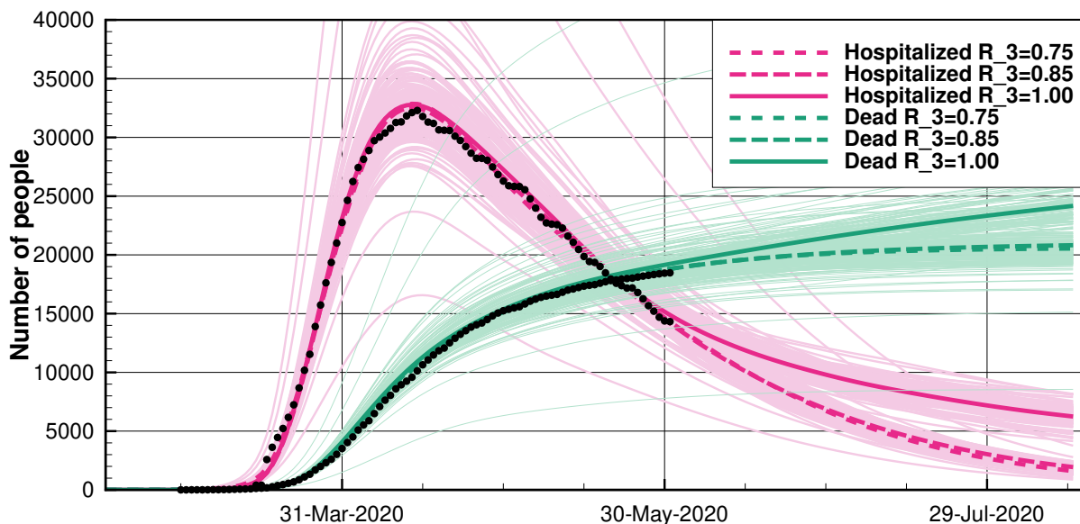
FIGURE 12. France: The plot presents forecasts of the reference case with three distinct scenarios after intervention setting the reproduction number to R_3 = 0.75, 0.85, 1.00 . We have plotted the posterior values for the number of deaths at hospitals (green lines), and the hospitalizations (red lines), together with the first hundred realizations for each case.
