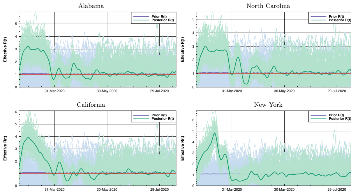
FIGURE 19. US Case 1: Large uncertainty in R(t)
