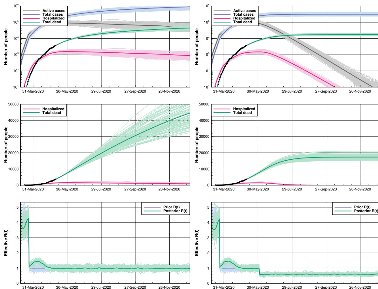
FIGURE 14. Brazil: The figure shows the simulation of the COVID-19 evolution in the São Paulo Brazilian State. In the left plots, we show a neutral case where the reproductive number R(t) \sim 1.0 with a standard deviation of 0.1 for the prediction. The right plots present a stable situation where R(t) \sim 0.6 with a standard deviation of 0.06, after a second intervention.
