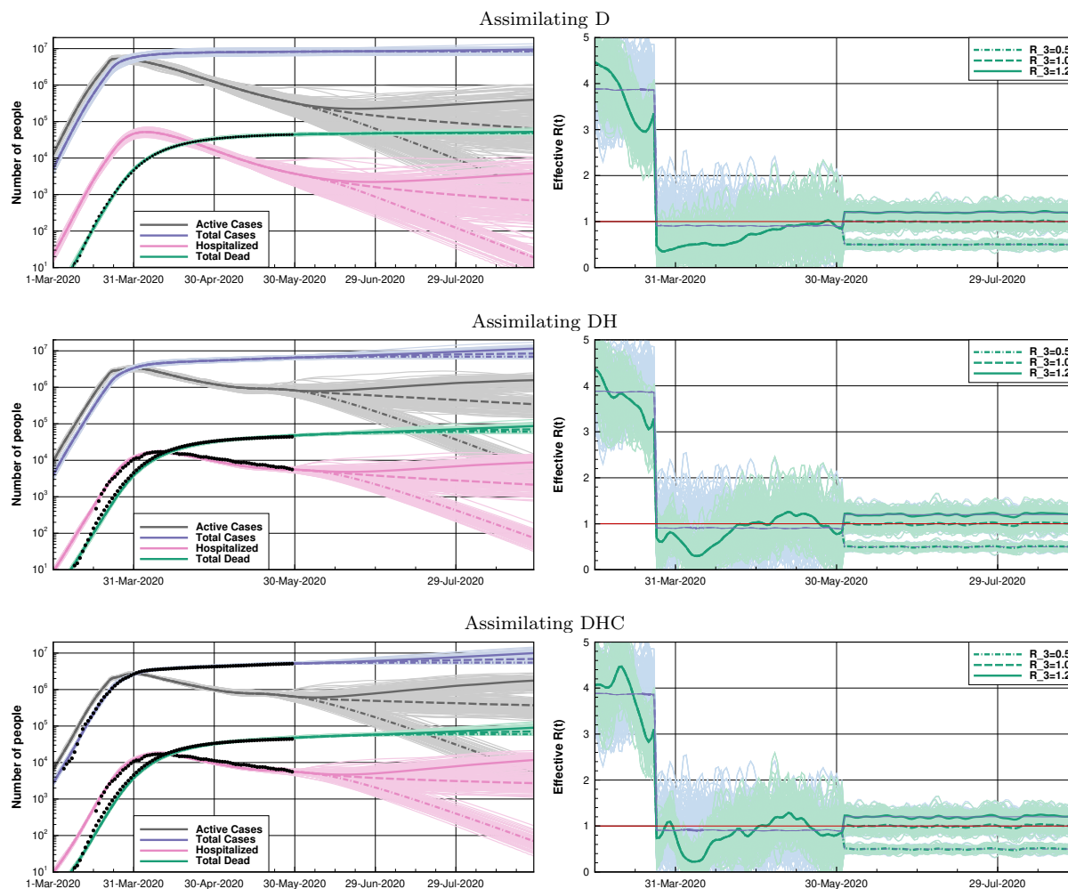
FIGURE 5. England. Left panels: ESMDA posterior estimates of the accumulated number of deaths (green), the daily number of hospitalizations (red), active (gray), and total cases (blue). Observations are displayed in black. Right panels: Prior and ESMDA posterior estimates of the effective reproduction number R(t) . Ensemble members (thin lines) and ensemble means (thick lines). Assimilation experiment D (top panels), DH (mid panels) and DHC (bottom panels).
