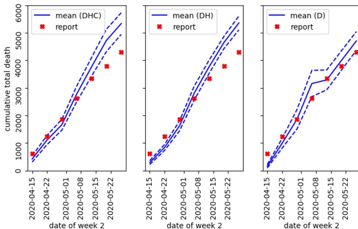
FIGURE 7. Quebec: The plots show verification of retroactive week-two forecasts for experiments DHC, DH, and D. For the predictions, issued one week apart, we show the mean estimate with the full line, and the dashed lines give the mean value plus or minus one standard deviation. We indicate the reported values with crosses.
