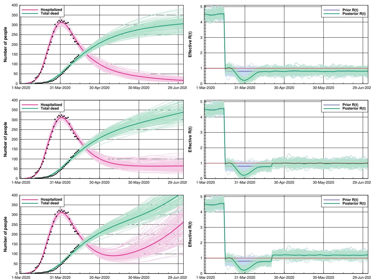
FIGURE 2. Norway: This figure presents a summary of scenarios related to opening up kindergartens and schools on the 20th of April. The left plots show the ensemble means and the 100 first ensemble realizations, for the number of hospitalized and the accumulated amount of deaths for different scenarios of future R(t) = 0.8, 1.0, and 1.2 . The right plots show the prior and posterior ensembles of R(t) .
