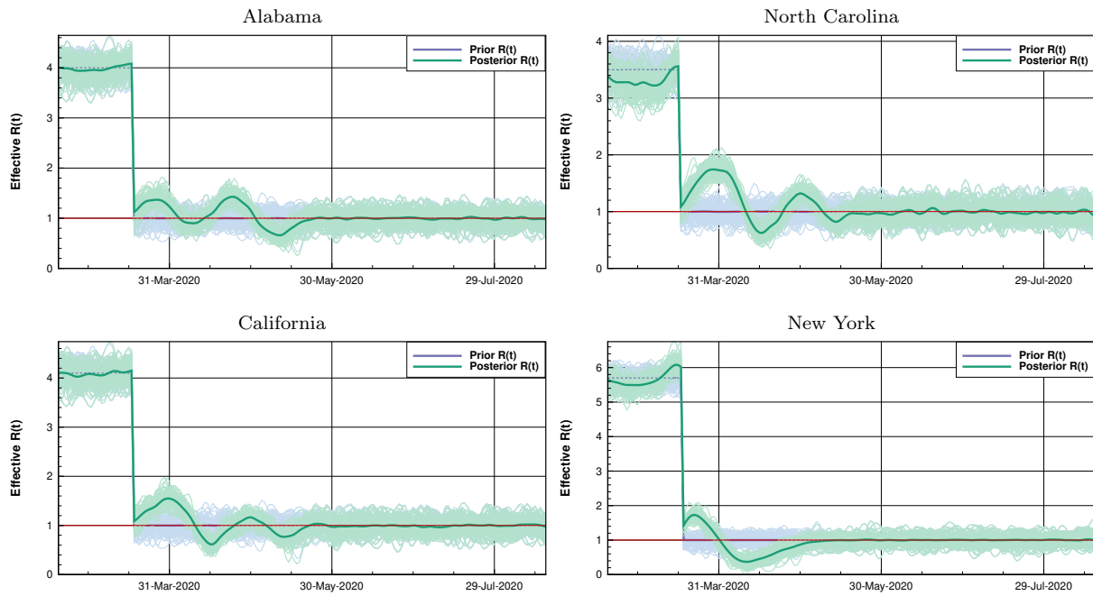
FIGURE 20. US Case 2: Assuming voluntary federal guidance was immediately observed by the citizens on March 16th.
