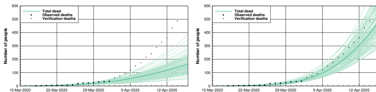
FIGURE 8. Quebec: The plots present verification of the week-two forecasts (retroactively) issued on April 1st for experiment D (left) and the experiment DHC (right). The solid line denotes the mean prediction. The reported values used to fit the model parameters are indicated with circles, while the triangles are the values used for verification.
