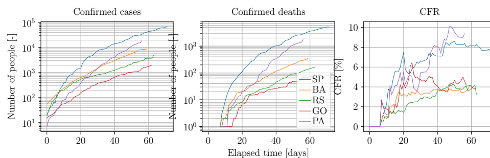
FIGURE 13. Brazil: The plots illustrate the evolution of COVID-19 in terms of the number of confirmed cases, deaths, and mortality rate (CFR), starting from the day of the first reported death by COVID-19. The reported states are São Paulo (SP), from the Southeast geopolitical region; Bahia (BA), from the Northeast; Para (PA), North; Rio Grande do Sul (RS), South; and Goiás (GO), Mid West. Each state represents a different evolution of the disease. We have shifted the curves in time to correspond to the first confirmed case.
