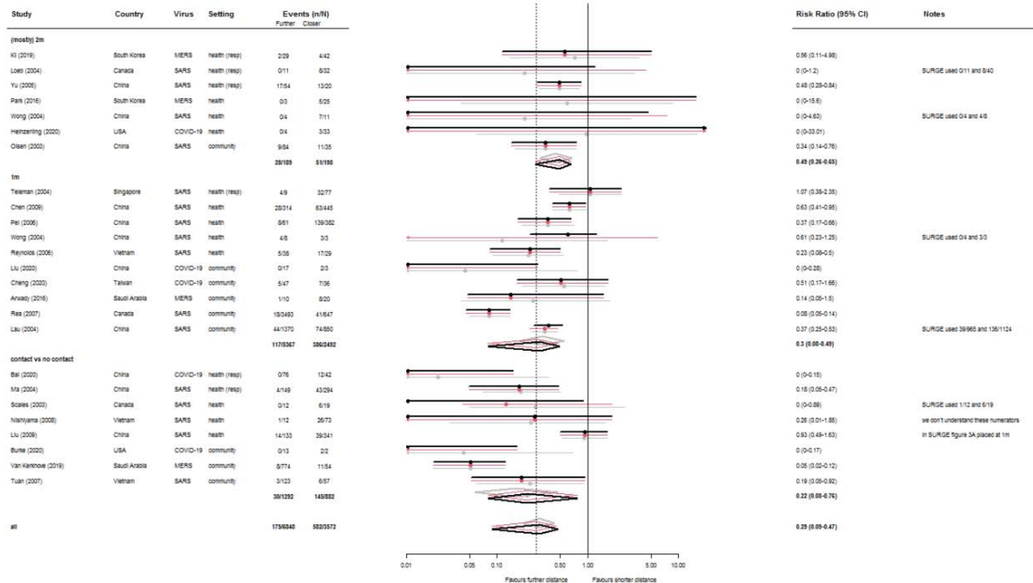
Figure 1: Forest plot of risk ratios estimated for each study, and groups of studies. Grey is estimates and 95% confidence intervals from the original SURGE[1] random effects meta-analysis. Red applies Tian's exact method [33] to this data. Black applies the exact method to the revised data described in this paper. The Notes column describes the differences between the datasets, and the RR column gives numerical estimates for risk ratios in the revised dataset calculated by the exact method. The setting column indicates whether the data were collected from a health care setting (with resp indicating respirators were in use there) or in the wider community.
