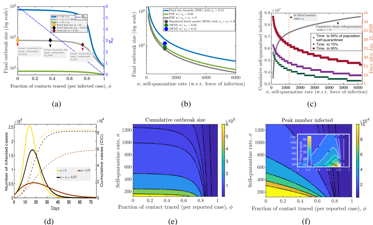
Figure 3: Sensitivity analysis of contact tracing and self-quarantine. All together the figures illustrate how contact tracing ( \phi ) has less impact on outbreak size ( \mathcal{C}_\infty ) than self-quarantine ( \sigma ) due to underlying concavity of their nonlinear relationships derived in final size formula (3). Fitted parameter values for China show that rapidly implemented lockdowns contained the outbreak, where a delay of 2 weeks in 95% of susceptible population being self-quarantined would result in a 10-fold increase in cumulative cases. Although contact tracing had little effect (2%) on final outbreak size, it “flattened the curve”, reducing peak infected by 34%. (a) Contact tracing (CT) proportion \phi versus outbreak size \mathcal{C}_\infty (nonlinear relationship) and reproduction number \mathcal{R}_0 (linear relationship) for 3 levels of self-quarantine (SQ) factor \sigma differing by order of magnitude of 10. (b) \mathcal{C}_\infty as a (nonlinear) function of \sigma for 3 levels of SQ susceptibility reduction \nu_q . (c) Total (final) self-quarantined individuals, along with time until 50%, 75%, 95% of population is self-quarantined as SQ factor \sigma varies. (d) Epidemic curve trajectories for 3 levels of CT proportion \phi marked in (a). (e,f) Contour maps of outbreak size and peak infected (with time to peak inserted) depending on CT proportion \phi and SQ rate \sigma .
