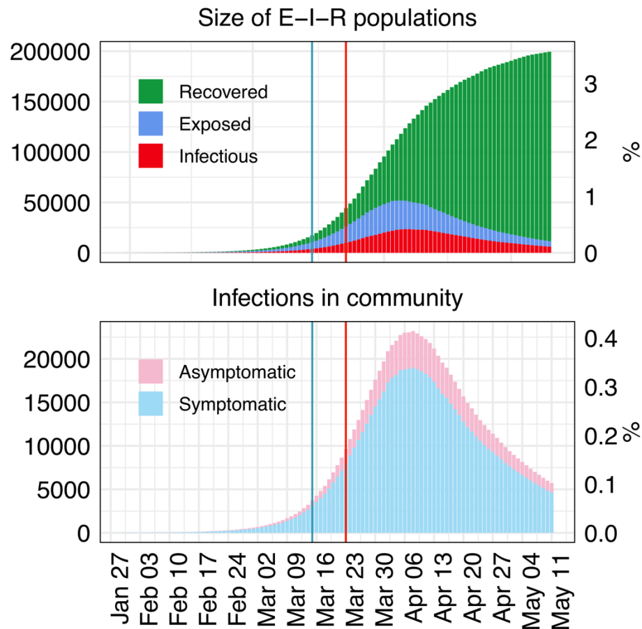
277 278 Figure 2: The predicted median size of the exposed (E), infectious (I) and recovered classes (R), along 279 with the size of asymptomatic and symptomatic individuals on each day in SW England until 11 th May 280 2020. Blue and red vertical lines represent the date the government introduced social distancing and 281 school closures/lockdown, respectively.
