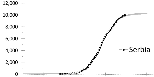
Confirmed cases M= 10,262 \alpha= 0.139 t_0= 15-04-20
