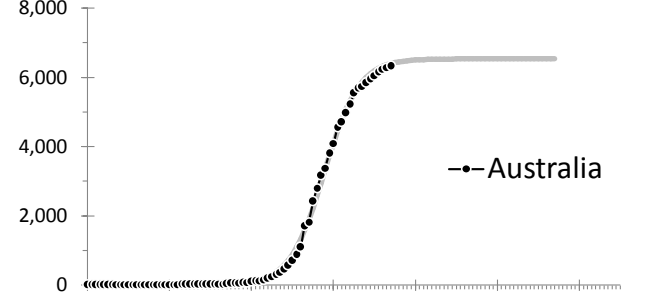
Confirmed cases M= 6,534 \alpha= 0.237 t_0= 27-03-20
