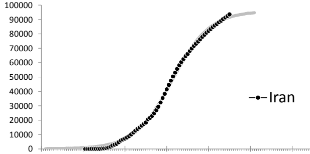
Confirmed cases M= 95,985 \alpha= 0.112 t_0= 01-04-20
