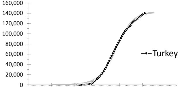
Confirmed cases M= 143,285 \alpha= 0.132 t_0= 15-04-20
