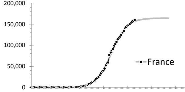
Confirmed cases M= 164,411 \alpha= 0.157 t_0= 1.8
