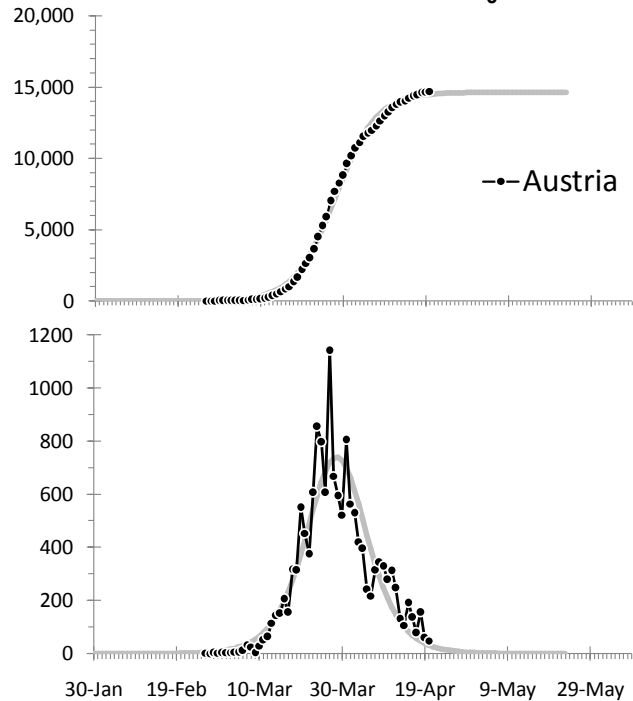
Confirmed cases M= 14,642 \alpha= 0.202 t_0= 28-03-20
