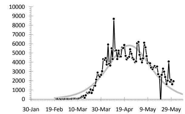
Confirmed cases M= 164,411 \alpha= 0.157 t_0= 1.8
