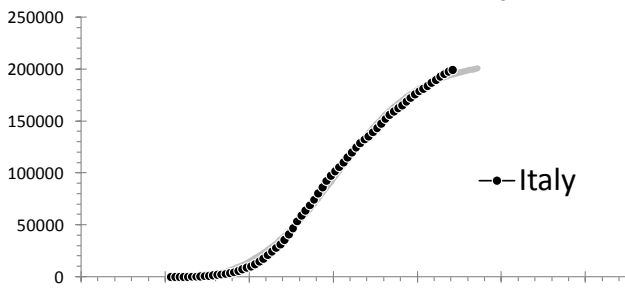
Confirmed cases M= 200,823 \alpha= 0.115 t_0= 31-03-20
