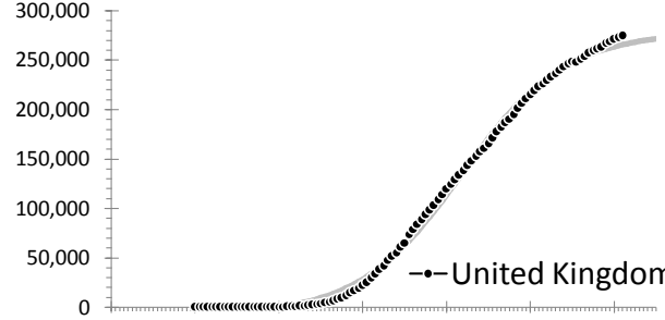
Confirmed cases M= 285,564 \alpha= 0.081 t_0= 22-04-20
