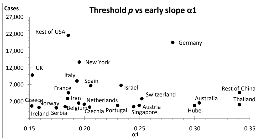
Figure 5. A scatter plot of the slope \alpha_1 of the early S-curves versus the threshold p ; high diffusion rates are preferentially associated with low thresholds.
