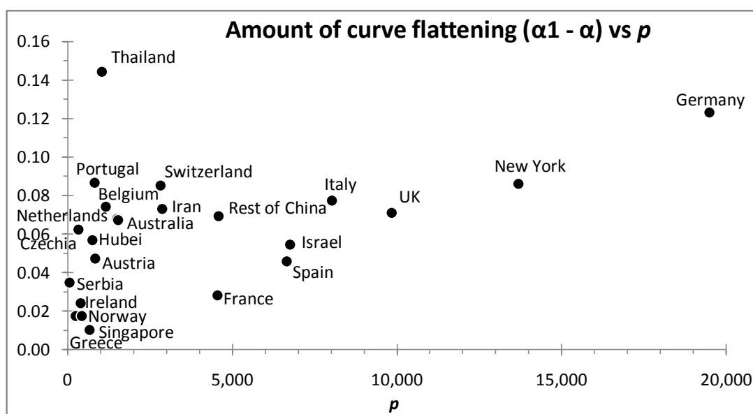
Figure 6. A scatter plot of the amount of curve flattening versus the lockdown threshold p ; the higher the threshold, the greater the flattening (and the distortion) of the S-curve.
