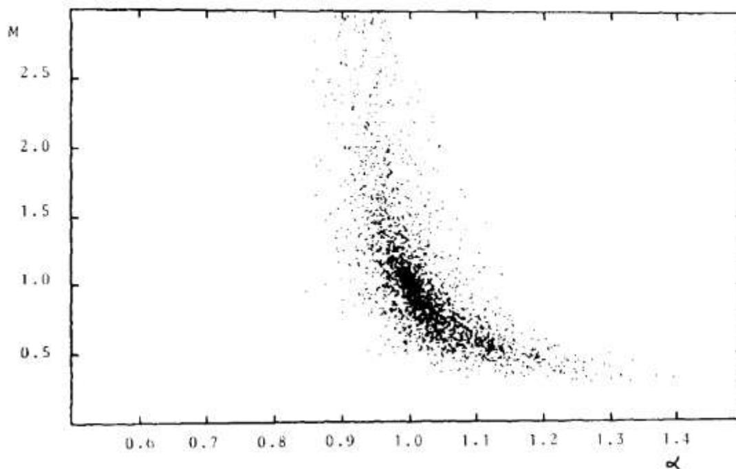
Figure 1. The correlation between M and \alpha reproduced here from the publication of Debecker and Modis. Every dot represents a logistic fit on simulated data (with added noise) that cover the early 20% of a logistic S-curve.
