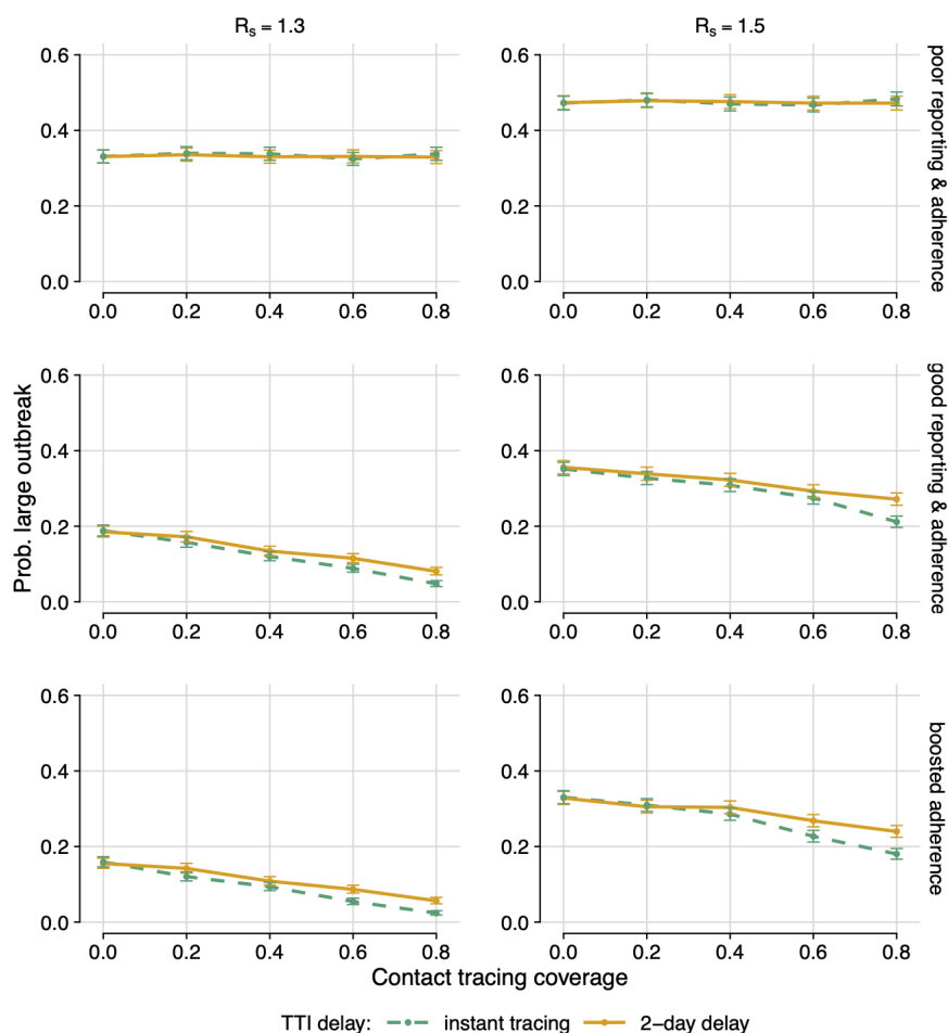
Figure 1: Probability of a large outbreak. Probability of a large outbreak (>2000 cases) for different Test and Trace compliance scenarios for instant testing and tracing (dashed, green) and a 2-day delay (solid, orange), assuming 95% test sensitivity. Poor reporting & adherence (top): 11.9% self-reporting; 18.2% isolation on symptoms; 10.9% isolation on tracing. Good reporting & adherence (middle): 50% self-reporting; 70% isolation on symptoms; 65% isolation on tracing. Boosted adherence (bottom): 50% self-reporting; 70% isolation on symptoms; 90% isolation on tracing. Left: R_s = 1.3 . Right: R_s = 1.5 . Error bars: 99% confidence intervals from output variation of 5,000 simulations. TTI = test, trace and isolate.
