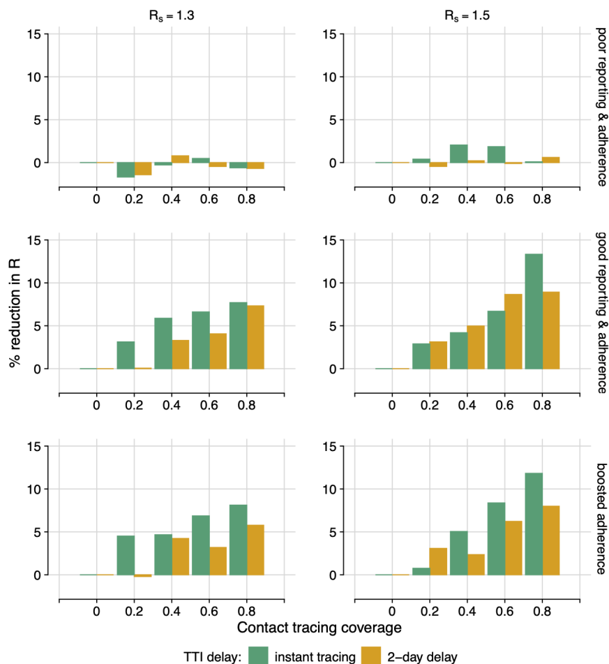
Figure 2: Contact tracing efficacy. Percentage reduction in the effective reproductive number, R , for different Test and Trace compliance scenarios. For instant testing and tracing (dashed, green) or a 2-day delay (solid, orange). Assuming 95% test sensitivity. Poor reporting & adherence (top): 11.9% self-reporting; 18.2% isolation on symptoms; 10.9% isolation on tracing. Good reporting & adherence (middle): 50% self-reporting; 70% isolation on symptoms; 65% isolation on tracing. Good reporting & high adherence (bottom): 50% self-reporting; 70% isolation on symptoms; 90% isolation on tracing. Left: R_s = 1.3 . Right: R_s = 1.5 . Combined results of 5,000 simulations.
