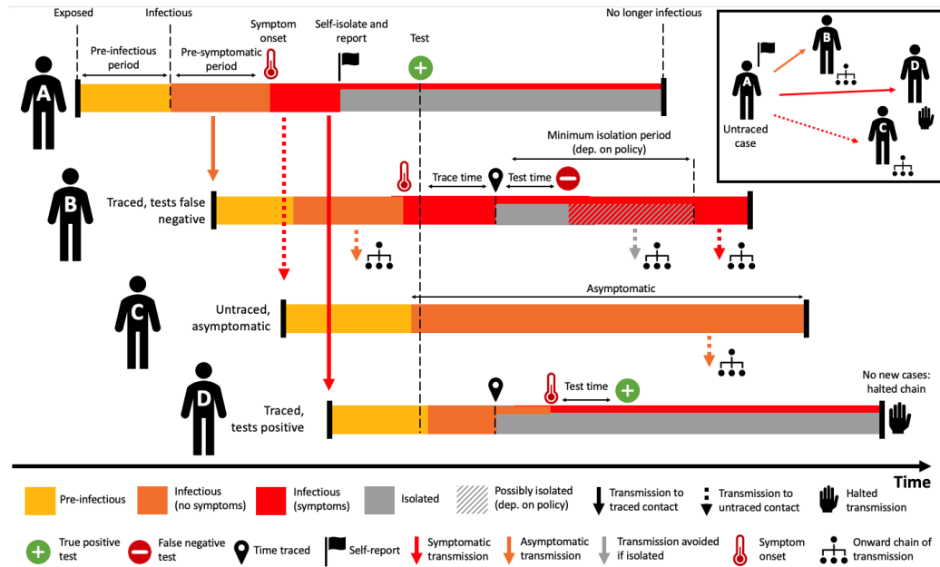
Figure 5: Contact tracing schematic. Overview of the contact tracing process implemented in our model. Person A isolates and self-reports to the contact tracing programme with some delay after symptom onset, by which time they have infected Persons B, C and D. When Person A self-reports they isolate and are tested, a positive result initiates contact tracing. Person B was infected by A prior to their symptom onset and is detected by tracing after some delay. After isolating they are tested, with a false negative result. This leads to B either a) stopping isolation immediately or b) finishing a minimum 7 day isolation period. Both may allow new onward transmission. Person C was infected by A but not traced as a contact. Person C does not develop symptoms but is infectious, leading to missed transmission. Person D is traced and tested. The test for D returns positive, meaning that D remains isolated, halting this chain of transmission.
