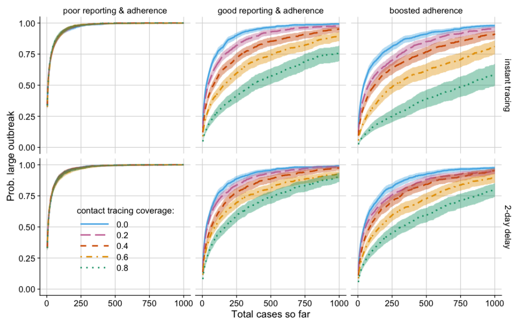
Figure 4: Outbreak thresholds. Probability of a large outbreak ( >2000 cases) by total number of cases so far (observed and unobserved). Sensitivity = 95%, self-reporting proportion = 50%, time to test from isolation = 1 day. Error windows: 95% confidence intervals from output variation of 5,000 simulations.
