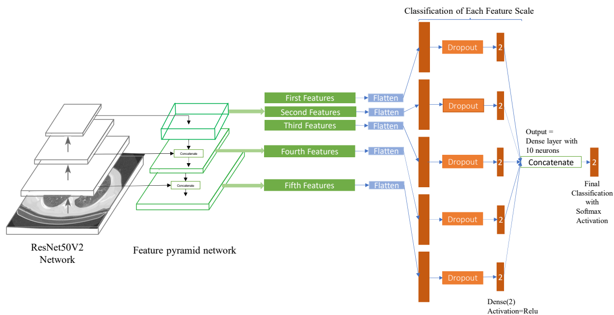
Figure 9: This figure shows the enhanced version of ResNet50V2 with feature pyramid network for classification.
