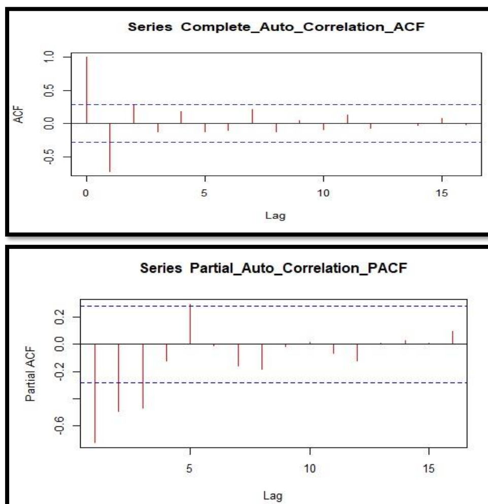
Fig. - The ACF and PACF plot for the determine the value of q and p for the model.
