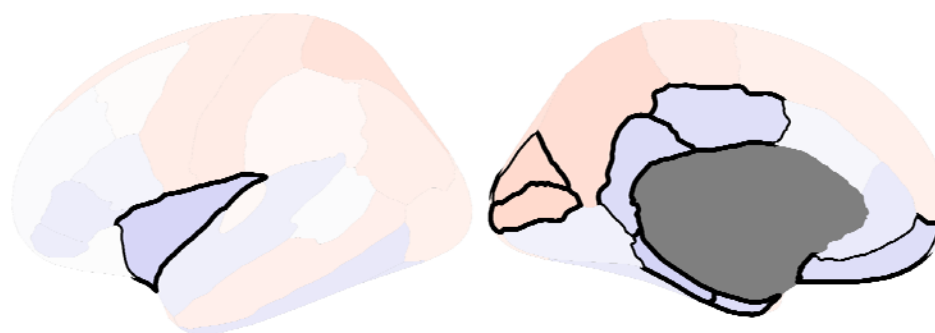
Figure 2. The effect of C4A expression on regional measures of (A) cortical surface area and (B) mean cortical thickness. The colors correspond to the standardized \beta (Std. \beta ) coefficient for each brain region from the linear regressions. Black demarcations around a brain region indicates that it passes the multiple comparisons–corrected significance threshold of FDR < 0.05 , with thicker lines indicating more significant findings.
