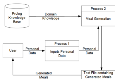
Fig. 2: Overall design of Experiments P_1 and P_2
