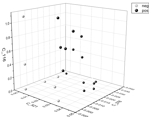
Figure 2 3D- scatterplot of signal intensities for cluster c_116, c_378 and c_521. White balls = Influenza-A negative, black balls = Influenza-A positive. The least significant cluster in the multivariate analysis is omitted, as it cannot be displayed in a 3D- diagram.
