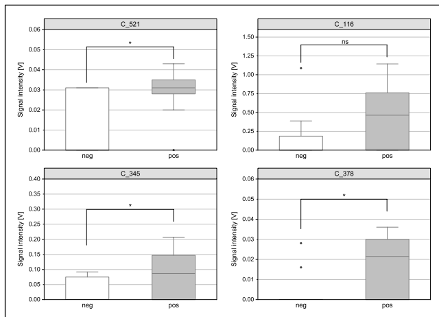
Figure 1 Boxplots of the peak intensities for the 4 most significant clusters C_116, C_345, C_378, C_521 in the multivariate analysis.
