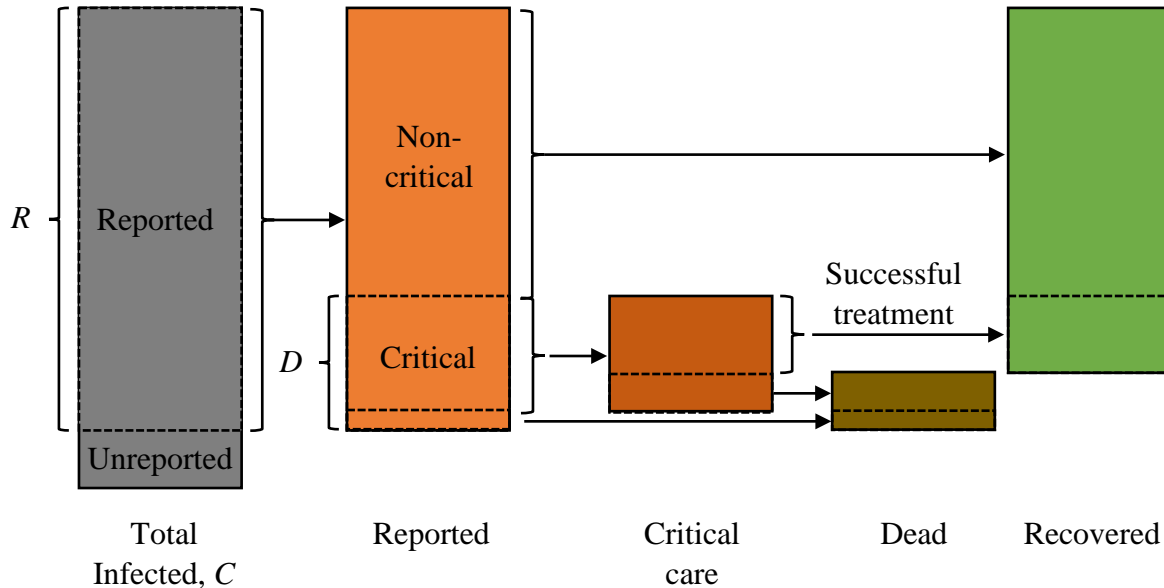
Figure 6. A diagram to illustrate the proportion of different groups at various stages of infection
