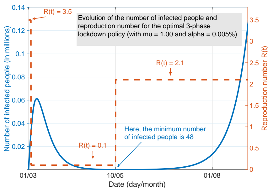
Figure 6: Optimal lockdown policy and corresponding dynamics for the Covid-19 epidemic.
