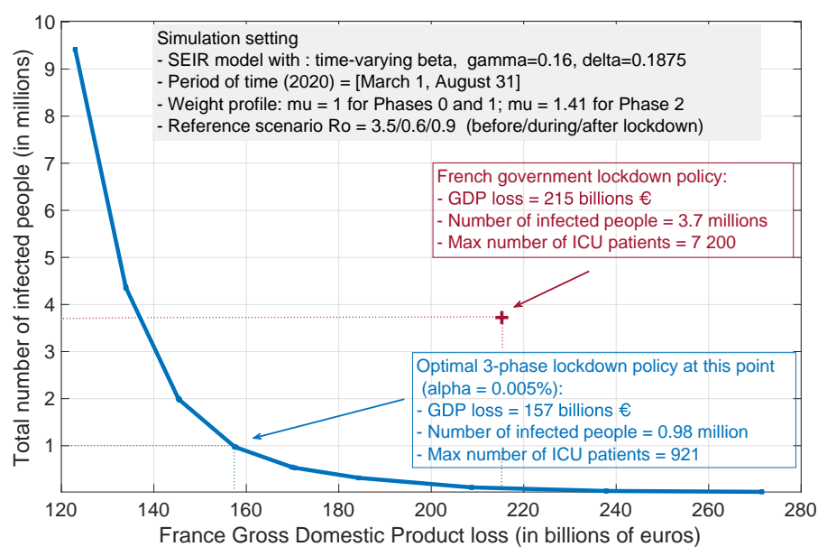
Figure 2: The curve represented here represents the pair best possible tradeoffs between economic cost (measured in terms of GDP loss) and health cost (measured in terms of the total number of infected people) that can be obtained (by choosing the best lockdown policy). In particular, with the assumed model, it is seen that it would have been possible to divide the number of infected people by about 4 and saving about 60 billions € in terms of GDP.
