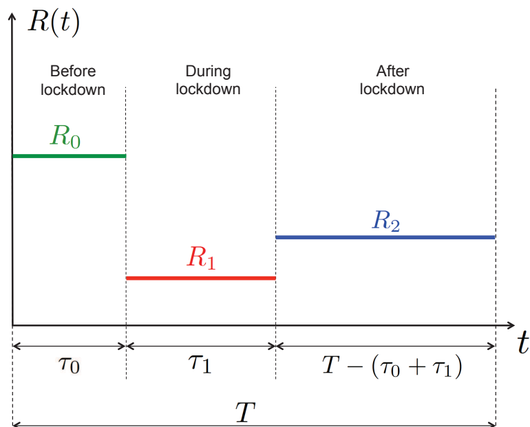
Figure 1: One of the goals of this work is to determine numerically, for a given tradeoff between health and economic aspects, the best 3–phase lockdown policy that is, the best values for \tau_0 , \tau_1 , R_1 , and R_2 (the epidemic time horizon T being given and the natural reproduction number R_0 being fixed).
