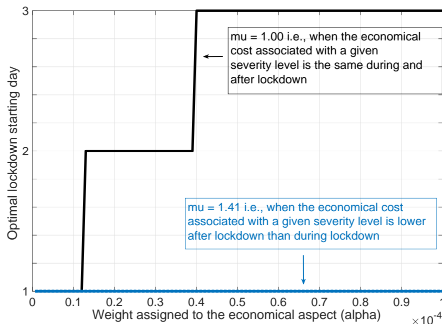
Figure 3: When economic losses are assumed to be uniform over time ( \mu = 1 ), there is some economic incentive to delay the lockdown, but this delay is seen to be at maximum 3 days. When economic losses are lower after lockdown than during it, the lockdown phase should always (up to the psychological dynamics) start as soon as possible (here on March 1).
