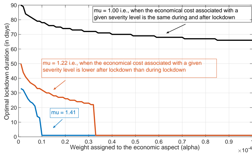
Figure 4: When economic losses are assumed to be uniform over time ( \mu = 1 ), it is optimal to have a long lockdown (typically between 60 – 80 days) whatever the tradeoff desired. But, if the economic losses of the third phase are less than during lockdown, the lockdown phase should be shorter or even absent.
