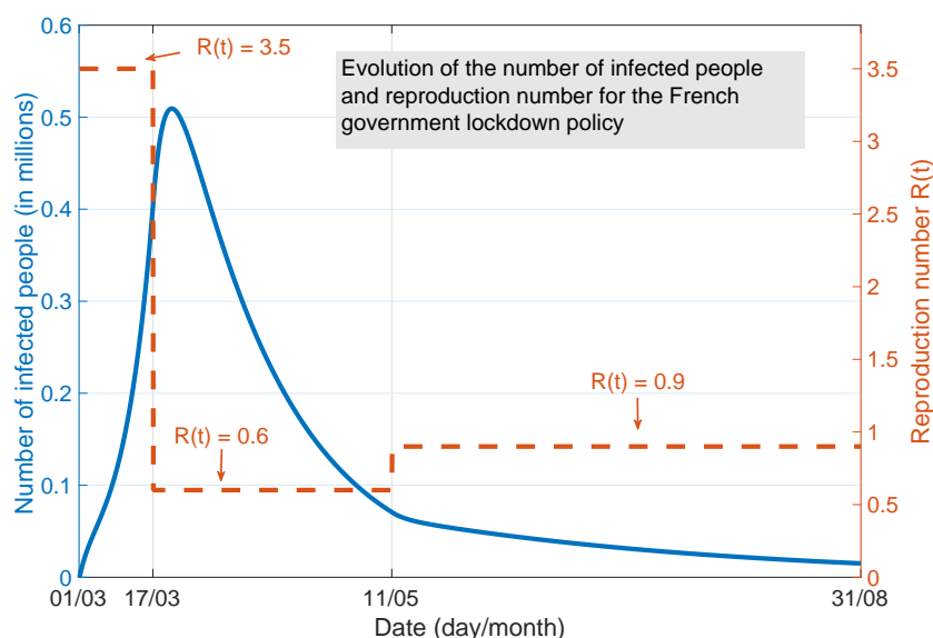
Figure 5: Evolution of the number of infected people and assumed reproduction number profile for the French government policy.
