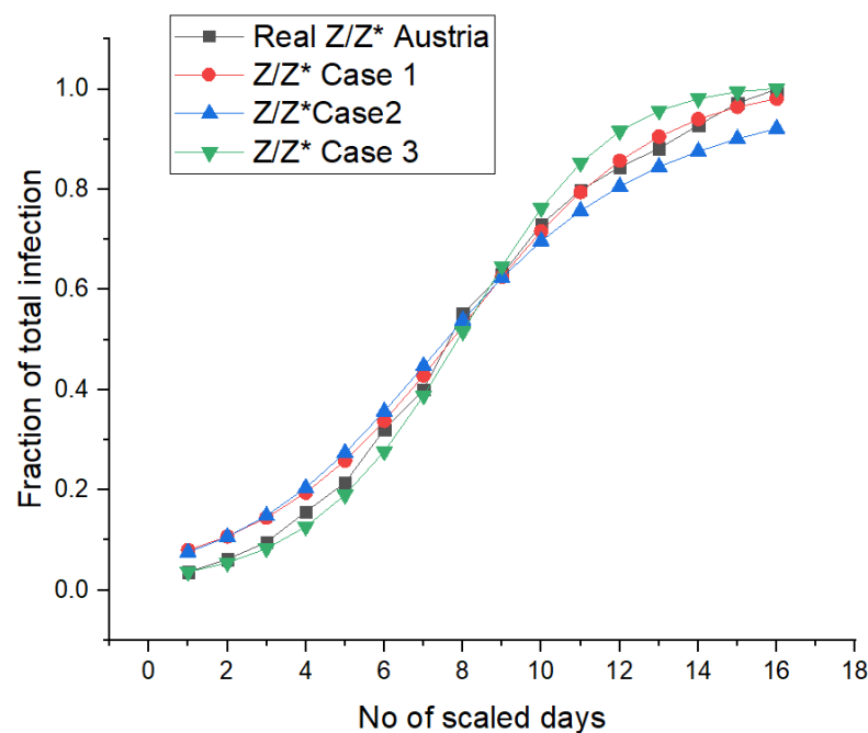
Fig 3: In above graph “Real Z/Z* Austria” represent the actual Z/Z* of Austria from 13 March to 12 April. The days are scaled accordingly. Case 3 is the same as Case 1 only the interaction parameter a=0.65 . Before 8 th scaled day case 3 overlaps with the actual data of Z/Z* and after 8 th day Case 1 overlaps. This clearly shows that the interaction parameter ‘a’ has reduced from a=0.65 to a=0.5 due to lockdown and governmental policies.
