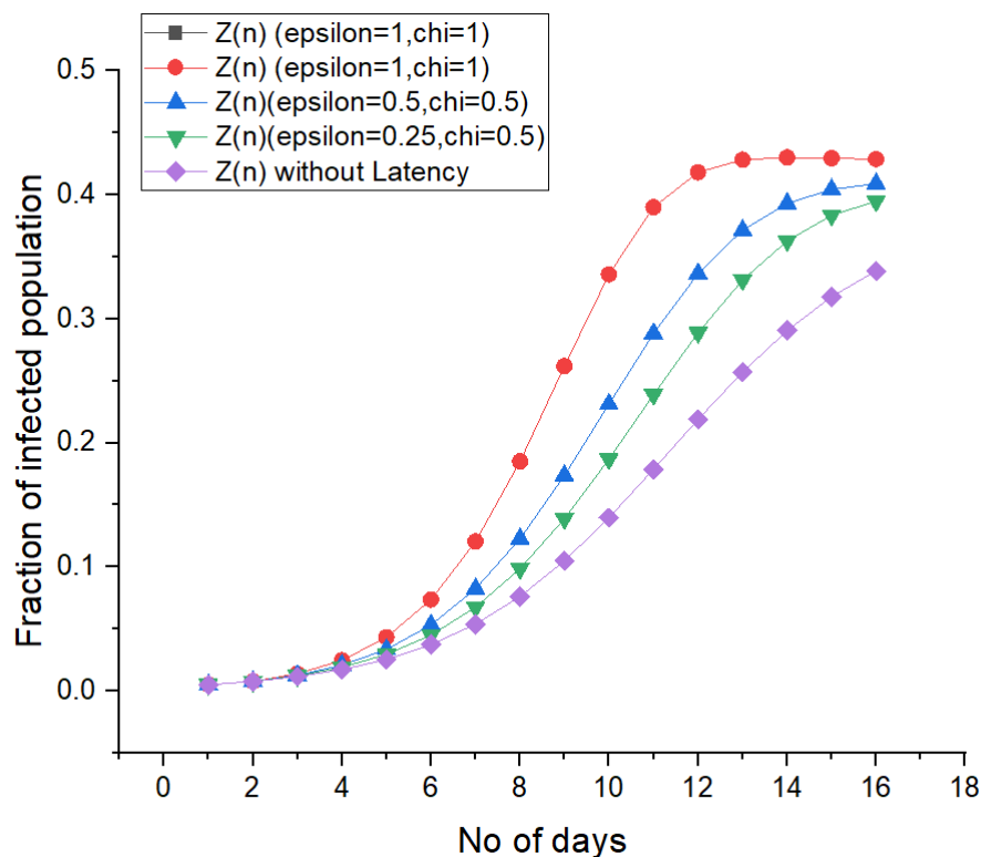
Fig 5: Above graph shows the effect of latency. When the saturation is more rapid, growth rate is high as compared to other two case when and .
