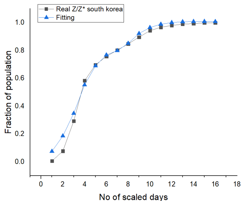
Fig 4: In above graph “Real Z/Z* South Korea” represents the actual value of Z/Z* of South Korea from 12 Feb to 14 April. Days are scaled accordingly. Before 4 th scaled day, parameters are difficult to predict due rapid fluctuations of parameters because of the Shincheonji gathering but it can be approximated to p=0.01 , a=0.9 , g=0.2 . On 5 th scaled day onwards probability of getting asymptomatics increased p=0.5 because of lockdown and government policies. On 6 th scaled day interaction parameter a decrease from ‘ a=0.9 to a=0.8 . On 7 th scaled day ‘ a=0.7 . Finally, on 8 th scaled day onwards interaction parameter ‘ a ’ decreases to a\approx 0.6 and remains constant afterwards.
