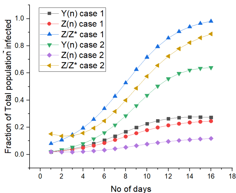
Fig 2: Case 1 and Case 2 are shown above. The parameters for Case 1 p=0.5, g=0.5, and a=0.5 . The parameters for Case 2 p=0.8, g=0.75,
