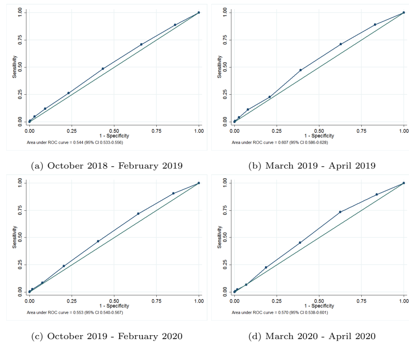
Figure 1: Area Under the Receiver Operating Characteristics (AUROC) and 95% Confidence intervals (CI) of suspected influenza case definition, Mexico 2018-2020
