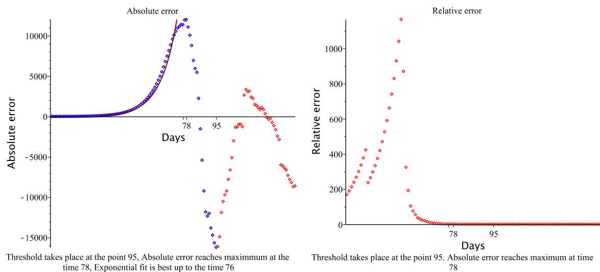
Fig. 2. Absolute and relative forecast errors.
