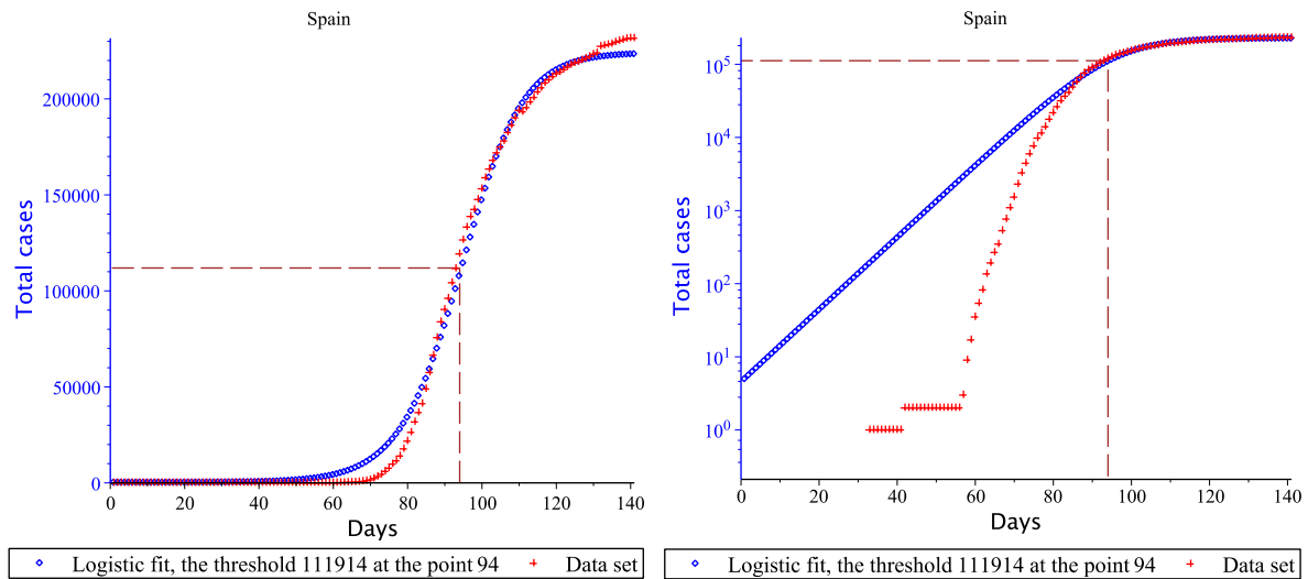
Fig. 1. The history of the epidemic in Spain. The red symbols indicate the total number of officially registered cases of infection by day, starting from the beginning of the epidemic in this country. The blue symbols represent the forecast line. The right graph is the same history presented in logarithmic scale.
