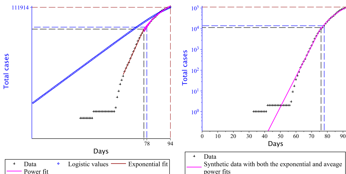
Fig. 3. Exponential and power approximation of input data. The graph on the right shows the possibility of replacing the monitoring data with approximating functions.
