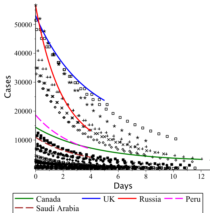
Fig. 5. Virtual time delay of epidemic monitoring data in Canada, the United Kingdom † , Peru, Saudi Arabia and Russia, which have crossed the epidemic threshold but have not yet reached its peak. We have used the same illustration as in Fig. 4 on the left as a background for visual comparison.
