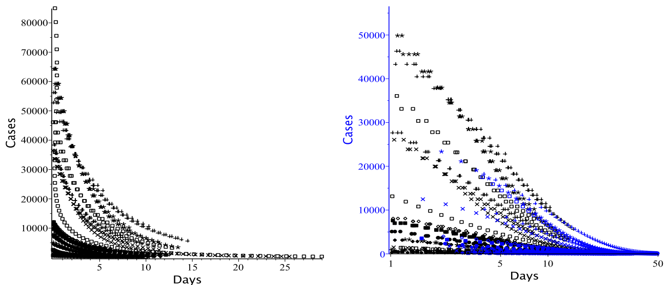
Fig. 4. Virtual time delay of monitoring data. The graph on the left shows the main part of the time delay calculated using a power-law approximation of the input data. In the illustration to the right of the main part, an insignificant part of the time delay, which is calculated using the exponential approximation of the monitoring data, is added.
