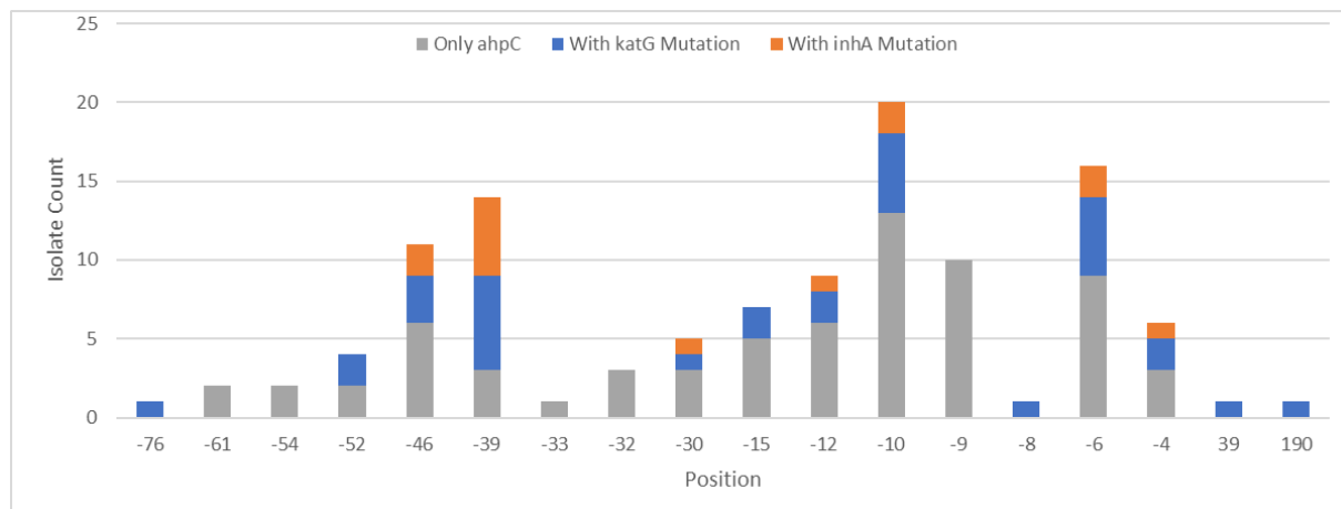
Figure 3: Mutations in intergenic region between the genes oxyR and ahpC (106bp in H37Rv genome positions 2,726,088 to 2,726,192). Negative positions are nucleotide positions relative to the start of the gene ahpC on the positive strand while positive positions are codon numbers in the gene's ORF. Blue bars indicate isolates that also harbor KatG mutations, while orange bars indicate isolates that also harbor inhA (promoter or gene) mutations. Grey bars indicate isolates that harbor no mutations in inhA (promoter or gene) or in KatG. Seven isolates had a mutation in katG and inhA .
