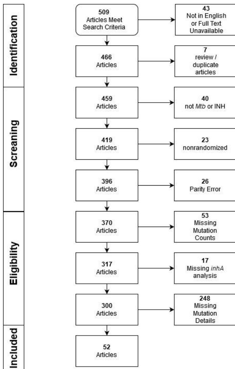
Figure 1. PRISMA Flow Diagram. Counts for exclusion criteria. Pubmed search term: (isoniazid OR inh) AND (resistance OR resistant) AND (mutations OR mutation) AND tuberculosis
