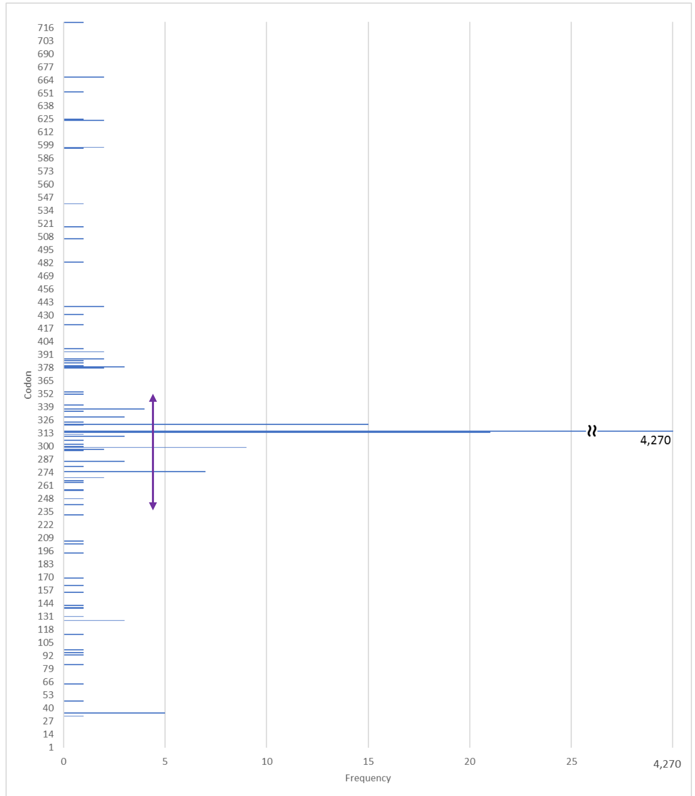
Figure 2. Frequency of mutations in katG observed in INH R clinical isolates.
