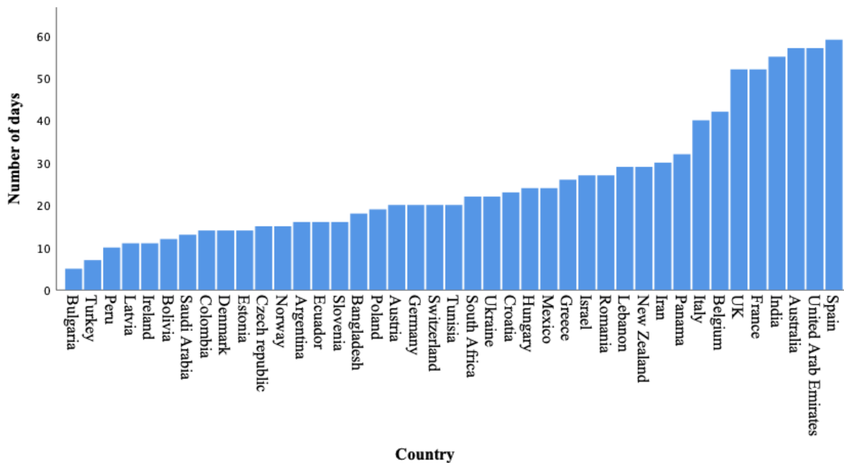
Figure 3: Number of Days Between Date of First Reported Case and Stay-at-Home Mandate per Country (n=41)
