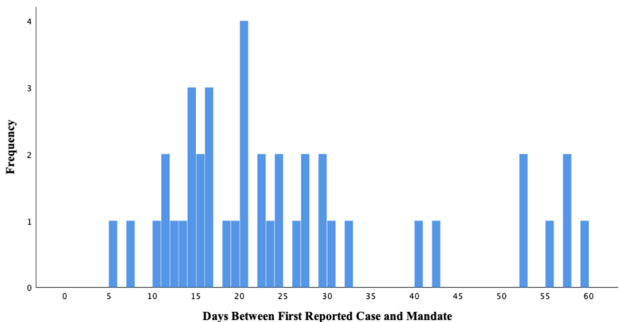
Figure 4: Distribution of the Number of Days Between Date of First Reported Case and Stay-at-Home Mandate per Country (n=41)
