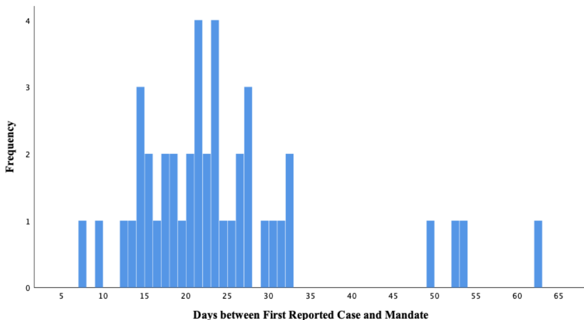
Figure 2: Distribution of the Number of Days Between Date of First Reported Case and Stay-at-Home Mandate per US State (n=43)
