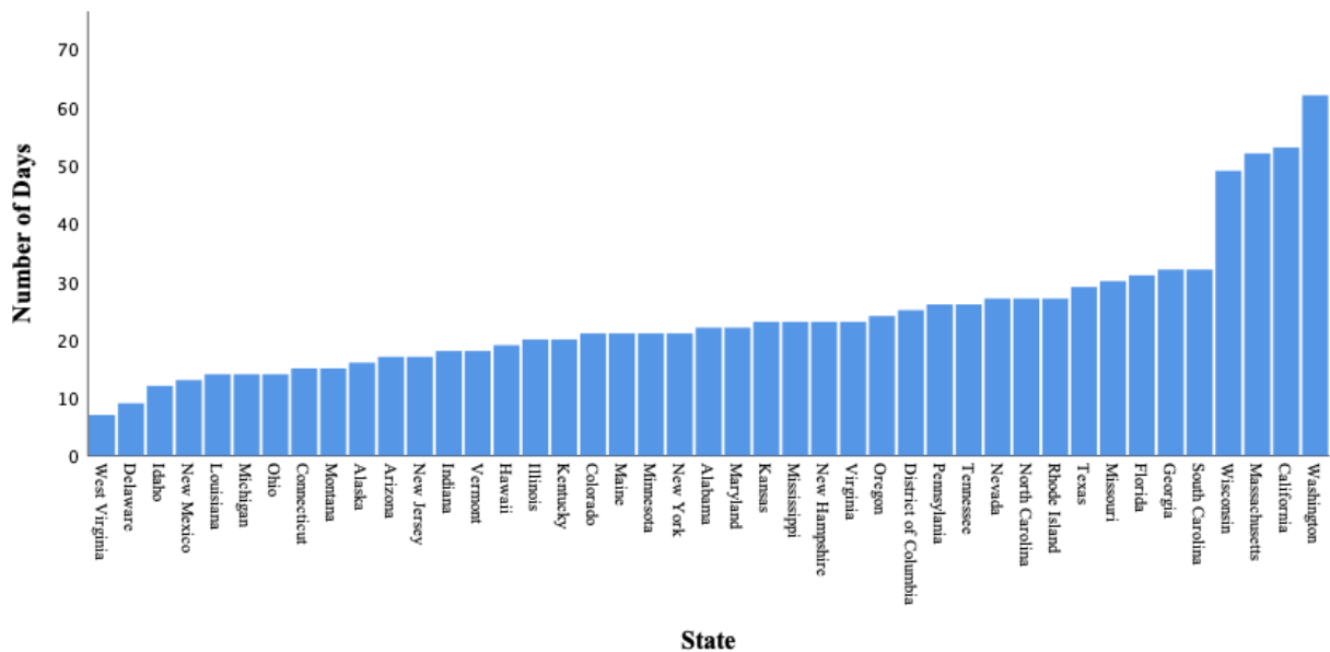
Figure 1: Number of Days Between Date of First Reported Case and Stay-at-Home Mandate per US State (n=43)
