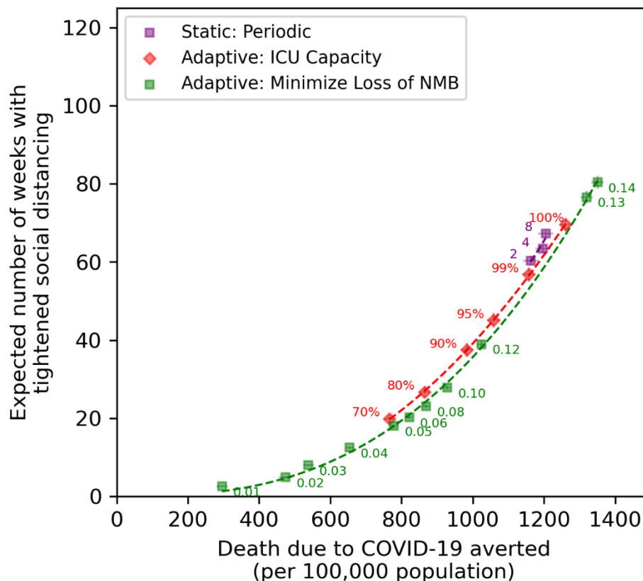
Fig. 2: Comparing the performance of difference physical distancing (PD) policies. The origin in this figure corresponds to a counterfactual scenario where PD is not used at all, which is expected to result in 1,391 deaths per 100,000 population. The curve ‘Static: Periodic’ corresponds to policies that recommend using PD every 2 weeks for 2 weeks, every 4 weeks for 4 weeks, and so on. The numbers on the red curve (‘Adaptive: ICU Capacity’) represent the probability that a COVID-19 patient who requires critical care would get admitted to ICU. The numbers on the green curve (‘Adaptive: Minimize Loss of NMB’) represent the trade-off thresholds of policies selected from Fig. 1A-B. The bars represent the 95% confidence interval of projections using 200 simulated trajectories. NMB: net monetary benefit.
