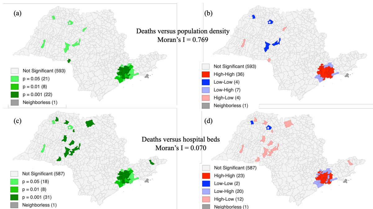
Figure 4: LISA's significant maps for the correlation between deaths and population density (a) and between deaths and availability of hospital beds (c), and LISA's clusters maps for the correlation between deaths and population density (b) and between deaths and availability of hospital beds (d). LISA's maps are based on data collected until May, 08 2020, for the State of São Paulo.
