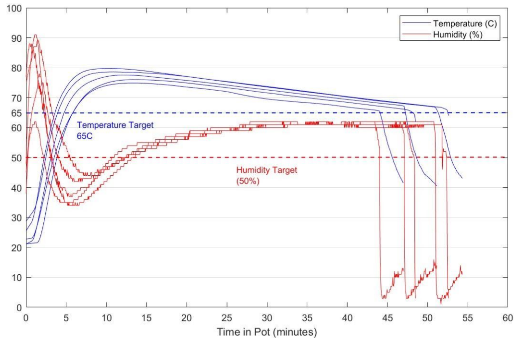
Figure 2: Temperature and humidity inside the container holding N95 respirators during the 5 treatment cycles after which they underwent filtration testing. Rapid decrease in humidity in the end is due to opening of the container at the end of the decontamination treatment.
