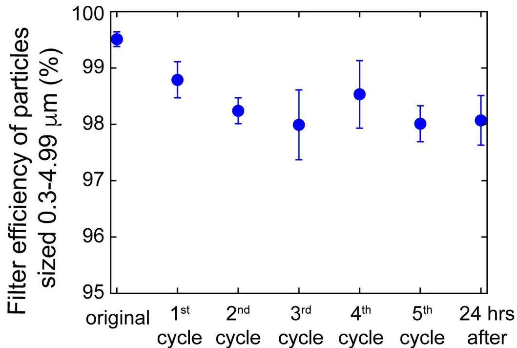
Figure 4: Filtering efficiency of particles sized 0.3-4.99 μm, at an intake rate of 2.83 l/min, of Kimberly Clark N95 respirators undergoing cycles of heat treatments using the method detailed in this protocol with 2L of boiled water.
