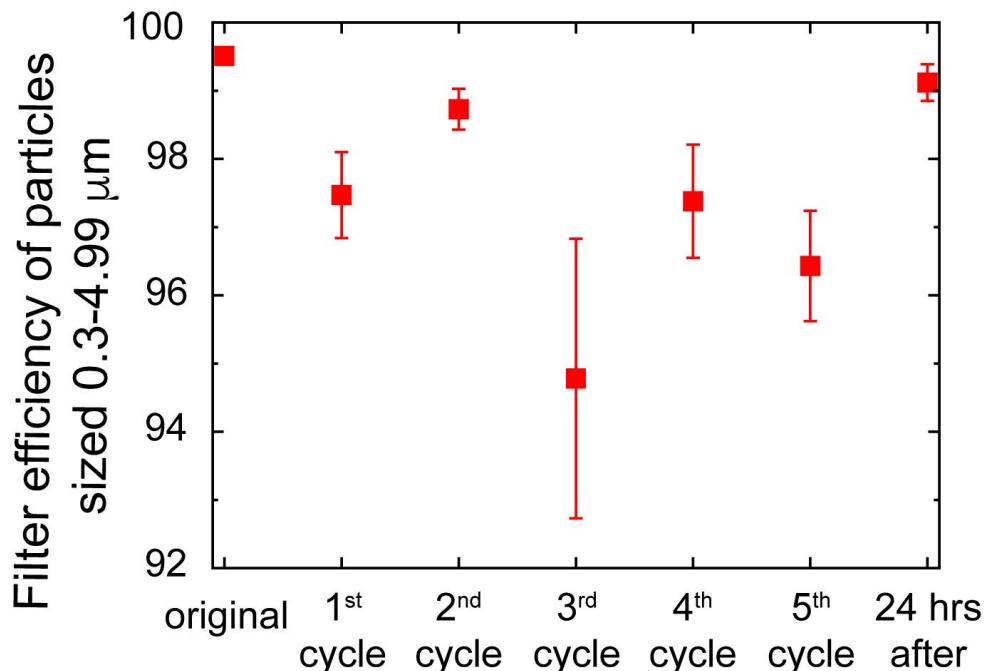
Figure 7: Filtration efficiency of particles sized 0.3-4.99 μm at an intake rate of 2.83 l/min as outlined previously, undergoing cycles of heat treatments while placed in Ziploc bags.
