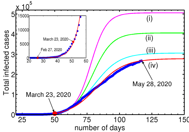
FIG. 2. Figure shows the two-phase evolution of the disease. The inset shows the good fit using Eq. (17) with the cumulative infected cases for the UK \bullet prior to March 23, 2020. Parameter values used are N_a(0) = 1.86 \times 10^5 , N_t(0) = 13 , \alpha_c p_c = 9.0 \times 10^{-6} , f_i p_i \beta_i = 1.205 \times 10^{-6} . Post lock-down period: The four curves (i-iv) correspond to the four iterations of N_a(0) values. (i) N_a(0) = 5.0 \times 10^5 , \alpha_s p_s = 0.0 , (ii) N_a(0) = 4.0 \times 10^5 , \alpha_s p_s = 1 \times 10^{-3} , (iii) N_a(0) = 3.0 \times 10^5 , \alpha_s p_s = 2.8 \times 10^{-3} , and (iv) N_a(0) = 2.75 \times 10^5 , \alpha_s p_s = 2.8 \times 10^{-3} . The initial value of N_t(0) = 5687 on March 23, 2020.
