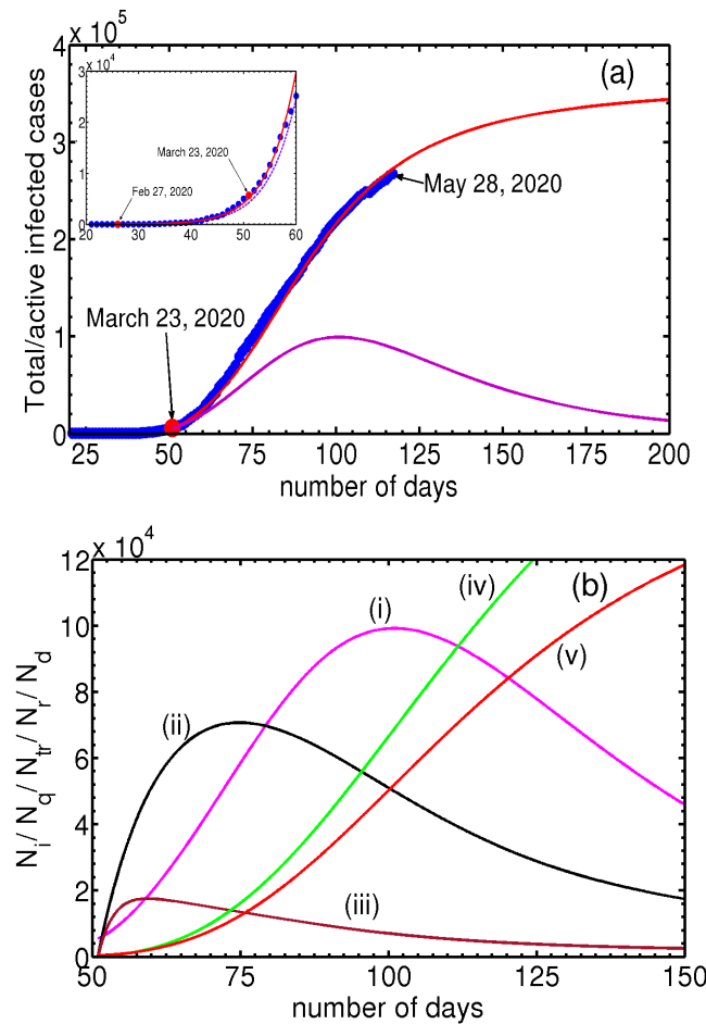
FIG. 4. (a) Inset: Plot of the total infected population (continuous curve), along with the UK data \bullet from February 27, 2020 till March 31. Also shown is the active infected N_i (dotted curve). Post Lock-down period: Plots of the total infected population (curve marked i) along with the corresponding data for the UK \bullet from March 23, 2020. Curve marked (ii) shows the active infected. (b) Plots of the infected (i), quarantined (ii), traced (iii), recovered (iv) and deceased (v), starting from March 23, 2020. The values of \alpha_s p_s = 8.0 \times 10^{-4} , \alpha_s p_q = 2.4 \times 10^{-2} and \alpha_t p_t = 2.0 \times 10^{-2} . Other parameter values are the same as given in Table I.
