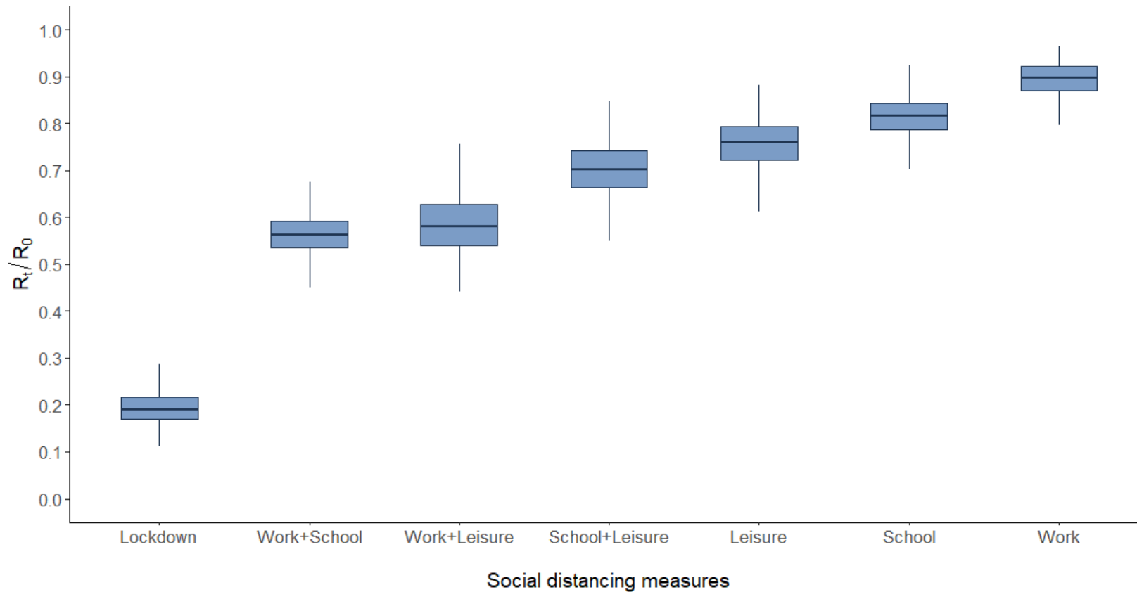
Figure 4. Estimated ratio R_t/R_0 to assess the impact of lockdown as well as the relative contribution of each measure or combination of measures as implemented during lockdown in Greece. A ratio of e.g. 0.80 corresponds to 20% decline in R_0 . The lowest ratio, corresponding to the period of lockdown, was obtained by comparing the social contacts data collected for the two periods (April 2020 vs January 2020). The other estimates were derived using the information from contact diaries in January 2020 corresponding to a regular school/working day and excluding or reducing subsets of social contacts at school, work home and leisure, based on what was observed during lockdown.
