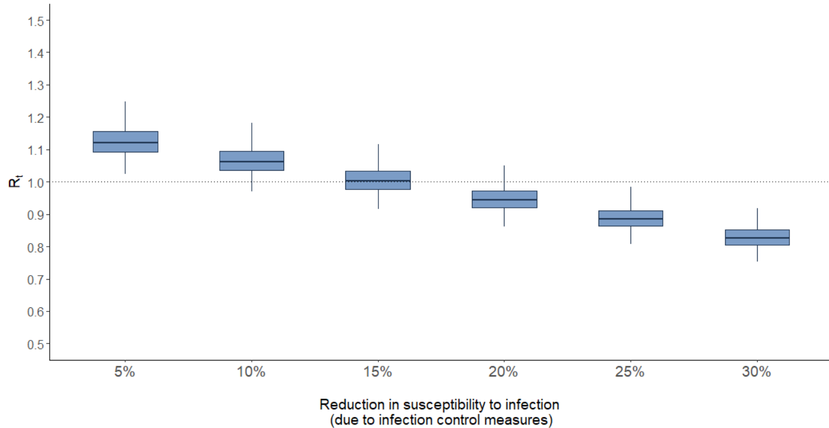
Figure 5. Estimated R_t following the partial lift of social distancing measures at the end of the first SARS-CoV-2 wave in Greece depending on the efficacy and adherence to infection control measures (hand hygiene, use of masks, keeping distances). R_t during lockdown was 0.46. For the partial lift of measures, we hypothesised a scenario where contacts at work, school and leisure activities will return to levels that are 50%, 50% and 60% lower compared to pre-epidemic levels, respectively.
