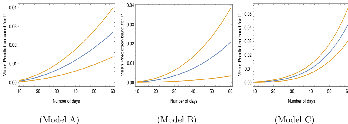
FIG. 2. Mean prediction band for I' at 90% confidence level for different models at T = 30^{\circ}\text{C} , H = 40\% and W = 10 \text{ Km/hr} . Blue line corresponds to best fit values.
