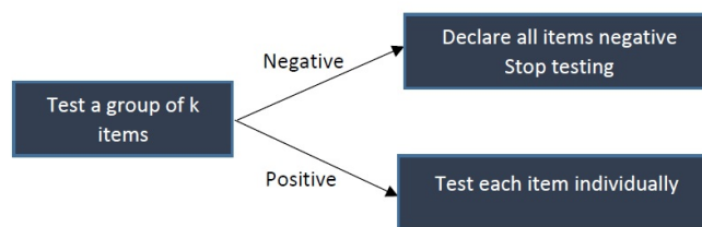
Figure 1: Process diagram of Dorfman's algorithm for pooled testing
