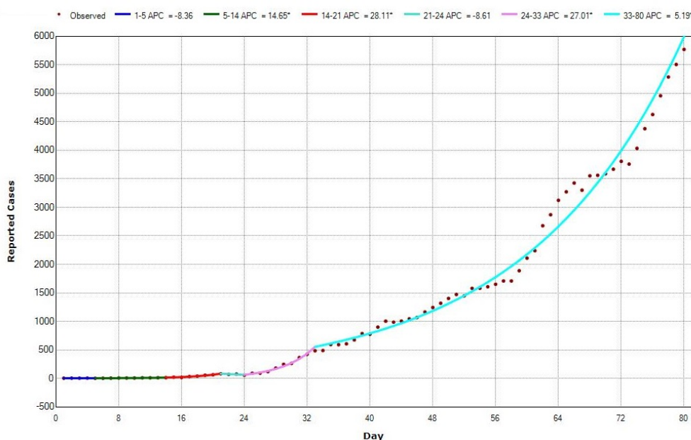
Figure 1 Joinpoint regression of daily reported confirmed cases of COVID-19 in India 1 March through 23 May 2020
