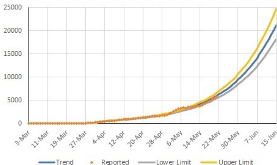
Figure 2 Forecast of COVID-19 cases in India up to 15 June 2020
