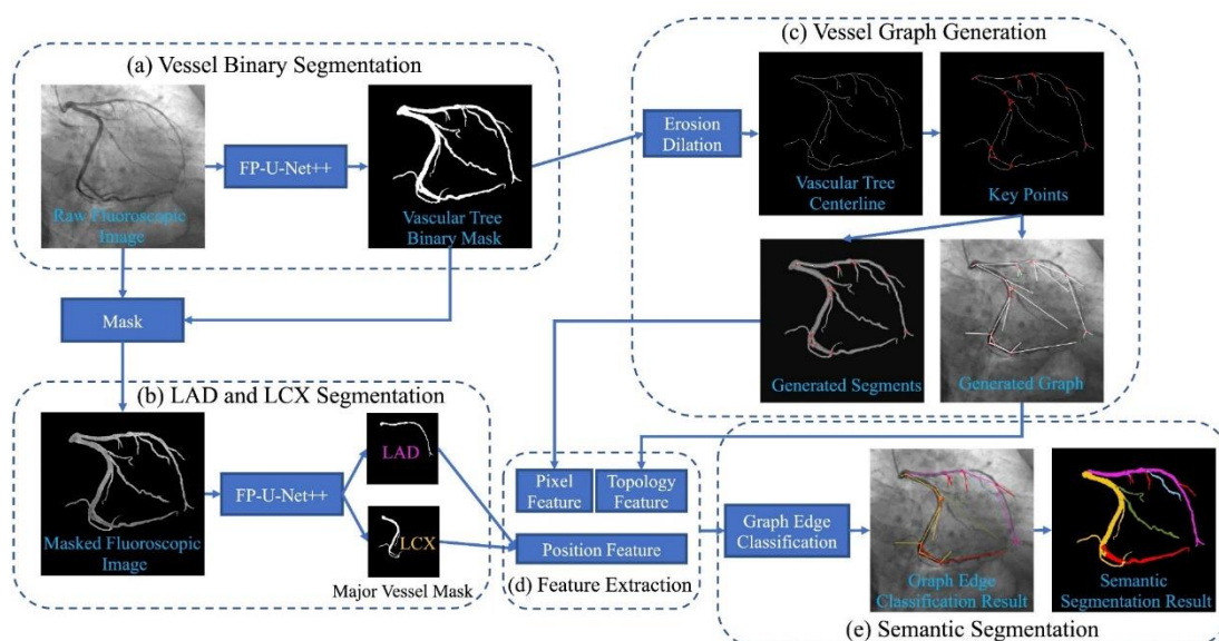
Fig. 2. Workflow of coronary arteries semantic segmentation.
