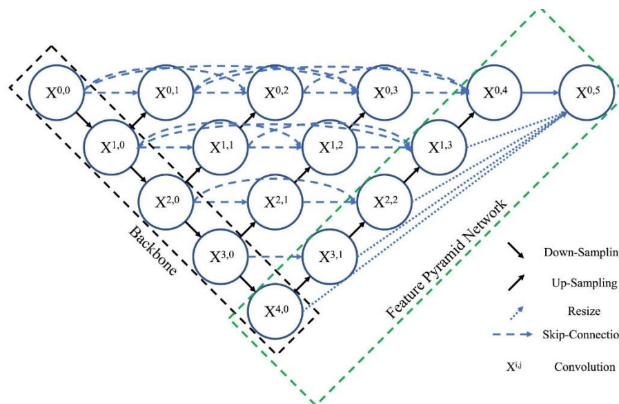
Fig. 3. Architecture of multi-output FP-U-Net++.
