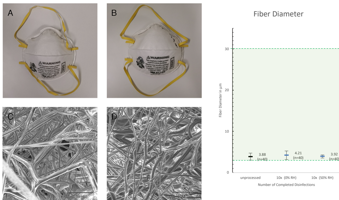
Figure 2: The effect of thermal disinfection on the structural properties of N95 respirators. (Left) The macroscopic and microscopic integrity of the respirator is preserved after repetitive disinfection. The upper left panels compare new (A) to ten times disinfected N95 respirators (B). Panels C and D show their filter layer in 650x magnification (SEM Image, Scale bar 50 \mu\text{m} , type 8110s, 3M, Minnesota, USA). (Right): Shown is the fiber diameter of unprocessed and ten times disinfected N95 filters (0% and 50%RH), with the fiber diameter range of new (untreated) 3M N95 filters shaded in green (9). Shown are the mean fiber diameters with 99% confidence intervals as error bars. Graphs are labelled with mean and sample size.
