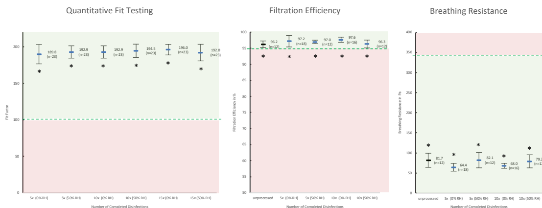
Figure 3: Function of thermally disinfected N95 respirators. Shown are the quantitative fit factors (left), particle filtration efficiency (centre) and breathing resistance (right) of thermally disinfected N95 respirators (0% and 50% RH). The US-governmental pass values for each test are indicated by a dashed line (11, 15, 16). Data are displayed as means with 99% confidence intervals and labelled with the mean and sample size. Groups that significantly exceeded the pass value are labelled with an asterisk ( * p < 0.01 ).
