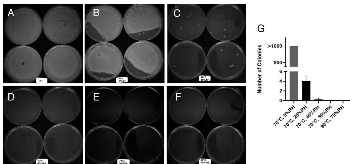
Figure 1: Bacterial inactivation in thermally disinfected N95 respirators. Panels A – F: E. coli colonies after 24h incubation at 37°C derived from inoculated N95 respirators that underwent treatment at different temperatures and humidity (A: incubation at room temperature (RT), B: 70°C / 0% relative humidity [RH], C: 70°C / 25% RH, D: 70°C / 40% RH, E: 70°C / 50% RH and F: 90°C / 70% RH as a control). Panel G: The E. coli colony count in
