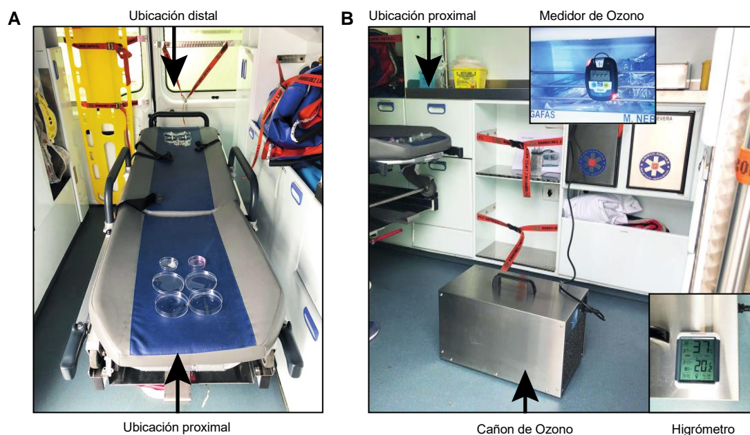
Figure 1. Environmental context and experimental setup. (A) Spatial location of the lentivector stocks and bacterial cultures on the stretcher within the ambulance, at the two sites (proximal and distal) referenced to the position of the ozone cannon. (B) Position of the ozone cannon within the ambulance. The ozonimeter was placed in the upper shelves as shown in the picture. The picture shows the moment in which the ozonimeter shows ozone levels superior than 10 parts per million (ppm), indicating the saturation of the ozonimeter and the warning lights. The hygrometer was introduced in the ambulance before and after the tests to register the humidity range during the experiments.
