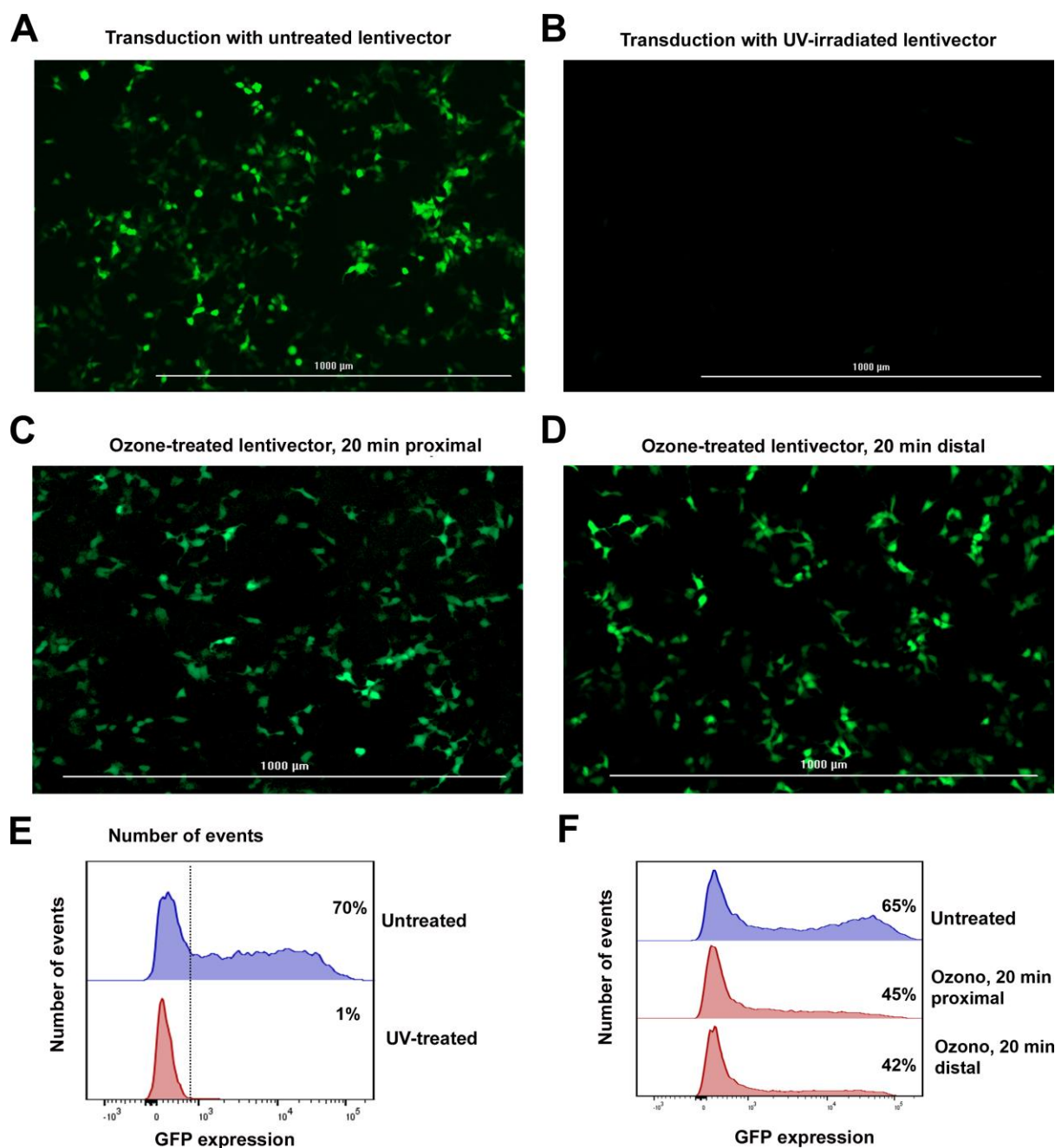
Figure 2. Effects of UV light and ozone treatments over the viability of lentivector preparations (A) Fluorescence microscopy picture of 293T cells transduced with an untreated control pSIN-GFP lentivector. GFP expression is indicative of infective capacities. (B) As in (A), but with lentivector stocks subjected to UV light treatments (UV-C, 20 min). The loss of viability is evident. (C) As in (B), but following a 20 min ozone treatment (>10 ppm) at the proximal location from the ozone cannon. (D) As in (C), but at the distal location. (E) Histograms with GFP expression from transduced 293T cells with the pSIN-GFP untreated lentivector stock, or previously treated with UV-light, as indicated. The vertical line indicates the separation between GFP positivity from negativity. Percentages of GFP-expressing 293T cells are shown within the graphs. (F) As in (E), but using lentivector stocks previously subjected to a 20 min ozone treatment at proximal and distal locations from the ozone cannon, as indicated.
