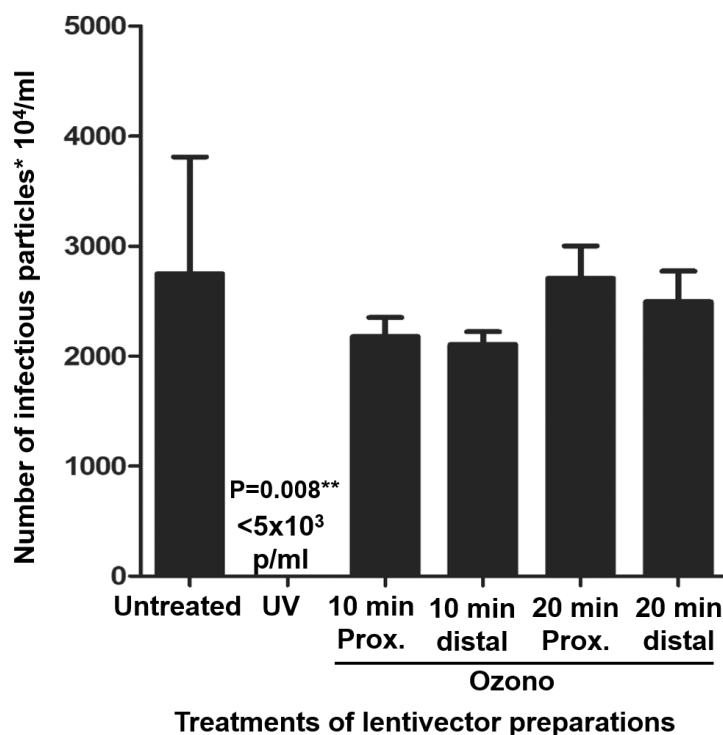
Figure 3. Titration of lentivector stocks after the treatments. Bar graphs presenting the titres of the lentivector stocks after the indicated treatments. Only the UV-light treatment significantly decreased the viability of the lentivector preparations. The detection limit of the titration technique is shown within the graph (<5 x 10 3 infectious particles/ml).
