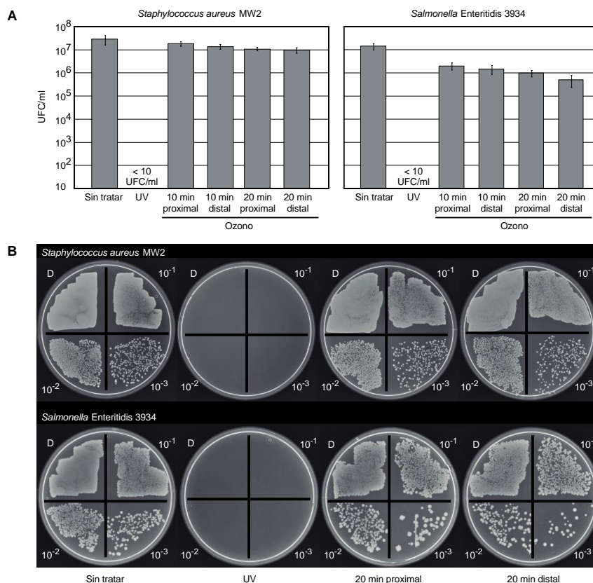
Figure 4. Effects of ozone treatments over the viability of S. aureus y S. Enteritidis . (A) Infectious colony-forming units per ml of viable S. aureus MW2 y S. Enteritidis 3934 cells following the indicated treatments. Means and standard deviation error bars are shown, from three independent experiments. The detection limit of the quantification technique is shown (10 infectious colony-forming units/ml). (B) Pictures of the culture dishes in which quantification of viable bacteria was performed, by 10-fold serial dilutions for each bacterial strain. The dilution of the bacterial preparation seeded in each quadrant is indicated. “D” indicates the undiluted bacterial suspension. Only the UV-light treatment significantly reduced the viability of both tested strains.
