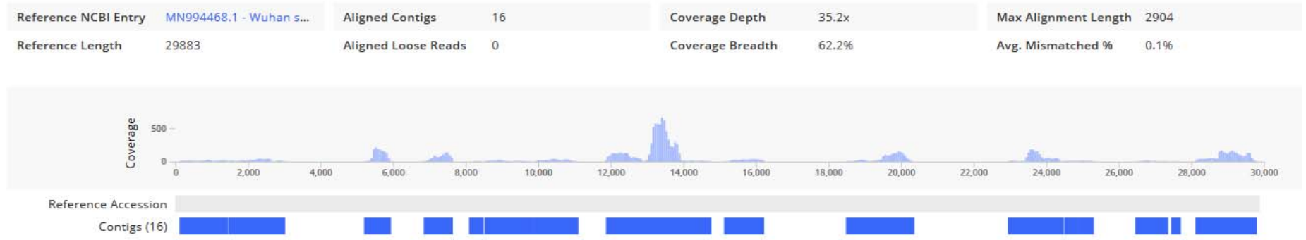
Supplementary Figure 1: A screen shot showing evidence of SARS-CoV-2 detection in metagenomics data using IDseq pipeline
