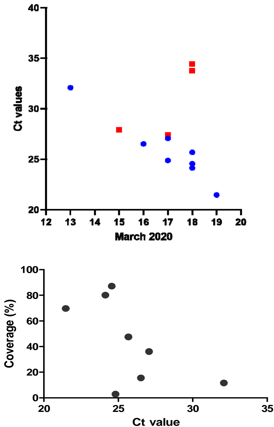
Figure 2: Distribution of Ct values of nasopharyngeal throat swabs of the study participant (A), and the association between Ct values and genome coverage of SARS-CoV-2 generated by mNGS (B)
