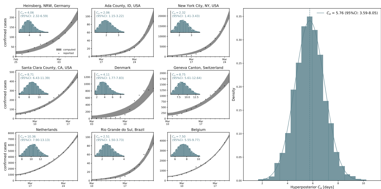
Figure 5: Hierarchical asymptomatic infectious period C_a estimation. Assuming an initial fixed reproduction number R_0 = 3.87 (95%CI: 3.01-4.66) [16], the simulation generates histograms of the asymptomatic infectious period C_a for each location based on the location-specific symptomatic fraction v_s . The black dots and grey regions represent the reported and simulated detected cases \hat{D}(t) and D(t) respectively. The hierarchical hyperdistribution for the asymptomatic infectious period results in C_a = 5.76 (95%CI: 3.59-8.09) days, right histogram.
