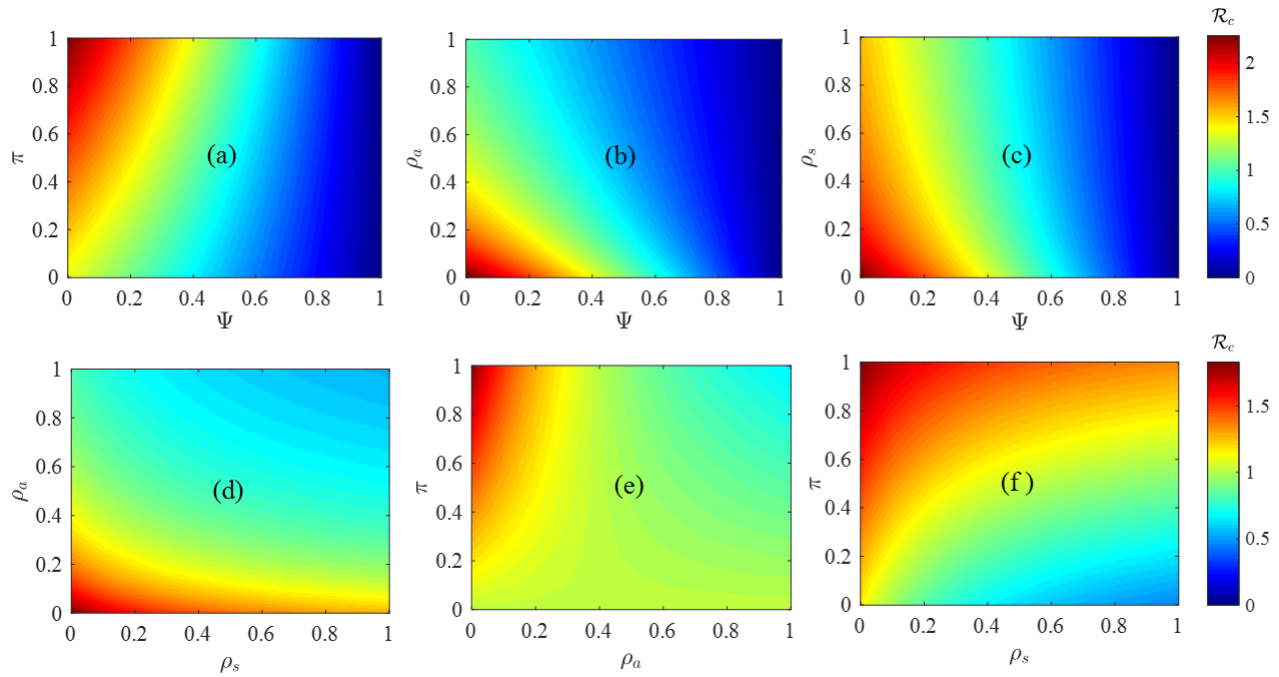
Fig. 5: Sensitivity of COVID-19 control reproduction number R_c , to different pairs of basic public health control measures. (a) Sensitivity of R_c to the proportion of exposed humans who develop COVID-19 symptoms at the end of the incubation period ( \pi ) and the reduction \Psi , in the disease transmission rate. (b) Sensitivity of R_c to the identification and isolation rate of asymptomatic infectious humans ( \rho_a ) and \Psi . (c) Sensitivity of R_c to the identification and isolation rate of symptomatic infectious humans ( \rho_s ) and \Psi . (d) Sensitivity of R_c to \rho_a and \rho_s . (e) Sensitivity of R_c to \rho_a and \pi . (f) Sensitivity of R_c to \rho_s and \pi .
