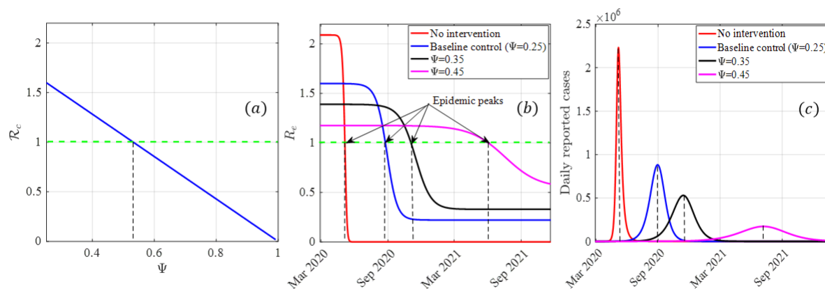
Fig. 4: Impact of control measures assessed through a reduction in the disease transmission term on the control reproduction numbers and the epidemic peak. (a) Plot of the control reproduction number R_c against the reduction in disease transmission due to the implementation of \Psi showing the threshold level of \Psi required to eliminate the disease. (b) Evolution of the effective reproduction number of COVID-19 in West-Africa for different values of \Psi . (c) Prediction and sensitivity of COVID-19 peak date to different values of \Psi . The initial conditions are S = 399, 386, 502 ; E = 1042 ; I_a = 14 ; I_s = 2 ; I_c = 1 ; R = 0 and the parameters are presented in Tables 1 and 2. The parameters for the initial period were used to plot the worst case scenario curves in the red (no control measure), while the parameters for the entire period were used for the other curves.
