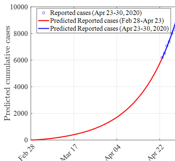
Fig. 3: Short term Prediction of the cumulative number of COVID-19 cases in West-Africa. The initial conditions are S = 399,386,502 ; E = 1042 ; I_a = 14 ; I_s = 2 ; I_c = 1 ; R = 0 and the parameters used for the simulations are presented in Tables 1 (entire period) and Table 2.
