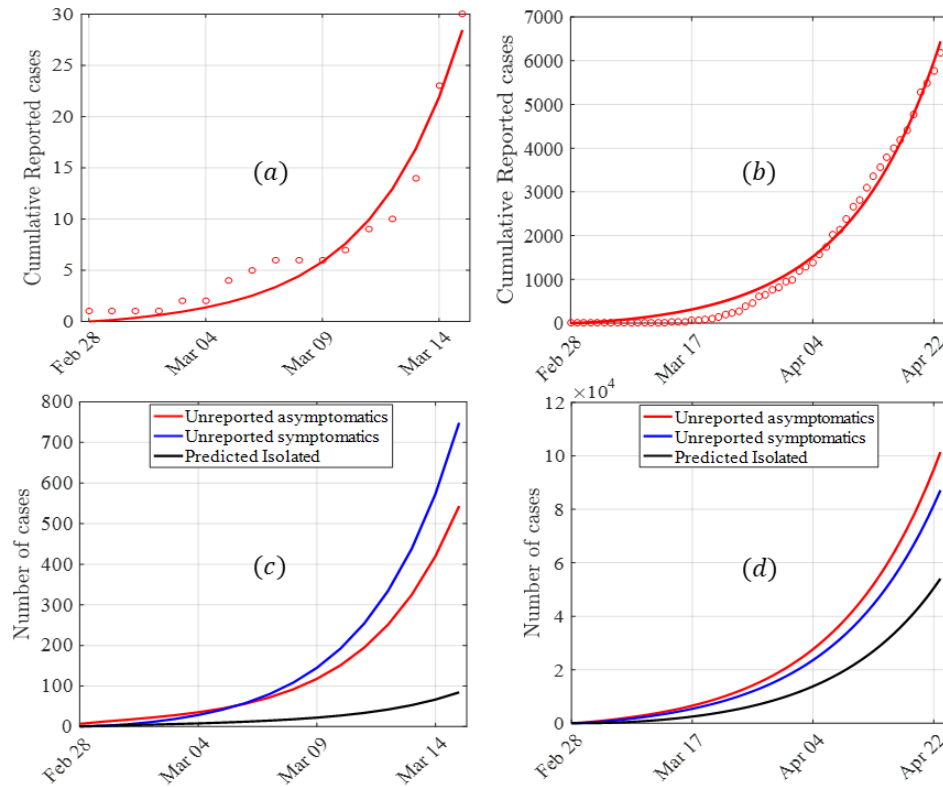
Fig. 2: Model fit and evolution trend of reported and unreported disease cases. (a) Model fit for the period from February 28-March 15, 2020, i.e., the first seventeen days when no control measures were applied. (b) Model fit for the period from February 28-April 24, 2020. (c) Evolution of predicted number of asymptomatic, symptomatic and isolated infectious cases period from February 28-March 15, 2020. (d) Evolution trend of predicted number of asymptomatic, symptomatic and isolated infectious cases for the period from February 28-April 24, 2020. The initial conditions are S = 399, 386, 502 ; E = 1042 ; I_a = 14 ; I_s = 2 ; I_c = 1 ; R = 0 and the parameters used for the simulations are presented in Tables 1 (entire period) and Table 2.
