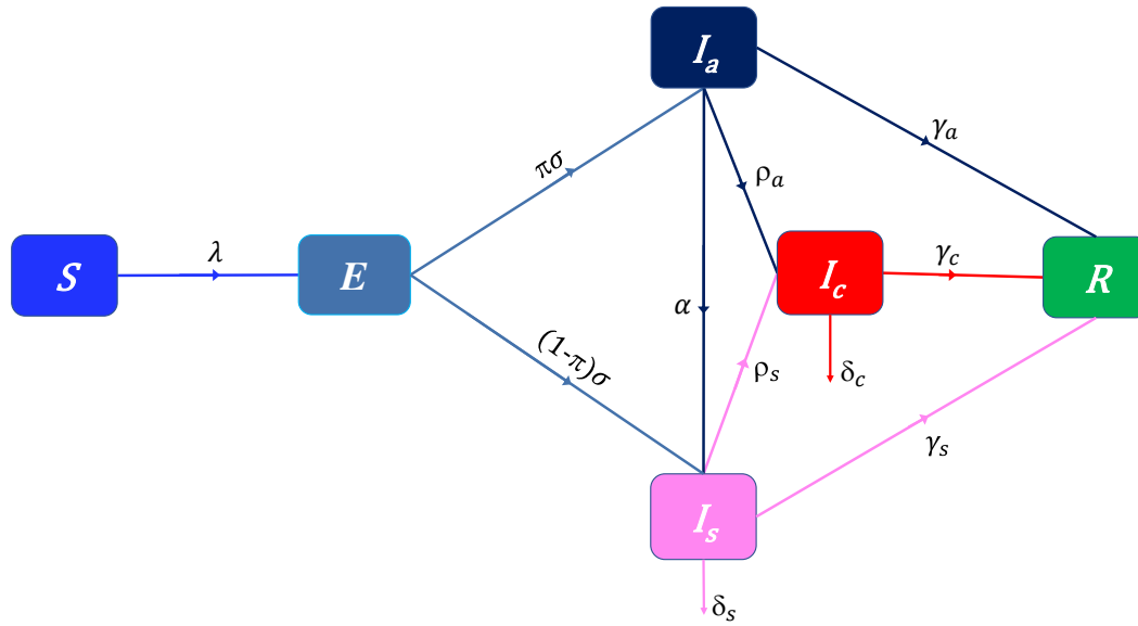
Fig. 1: Flow-chart of COVID-19 model showing the flow of humans between different compartments. The susceptible population is denoted by S , the exposed population is denoted by E , the infectious asymptomatic population is denoted by I_a , the infectious symptomatic population is denoted by I_s , the isolated infectious population is denoted by I_c , and the recovered population is denoted by R . The parameters of the model are described in the text.
