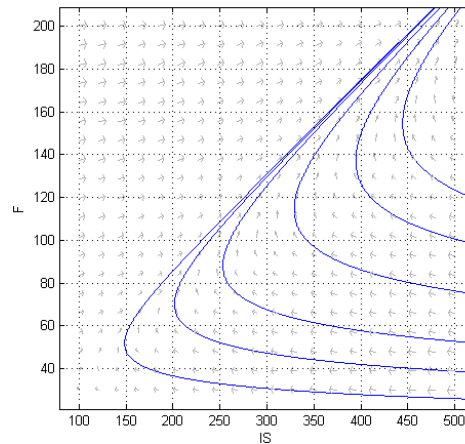
Fig.7. Transition diagram of interstate and foreigner population
