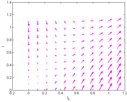
Fig. 8. Directional plot of Interstate population infected with Covid-19
