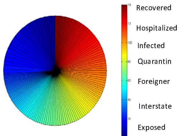
Fig. 13. Chaotic Diagram showing mortality rate of 2019-nCoV
