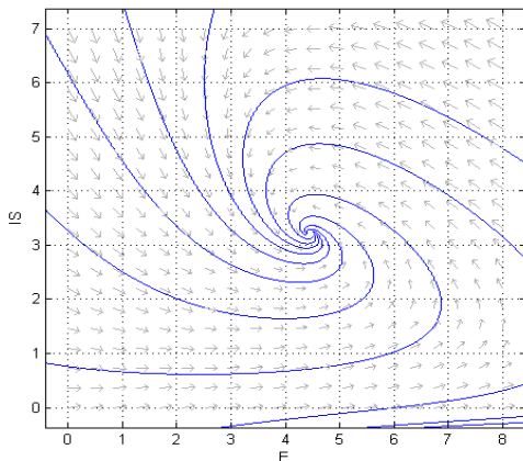
Fig. 4. Phase plot of interstate class when exposed to Covid-19
