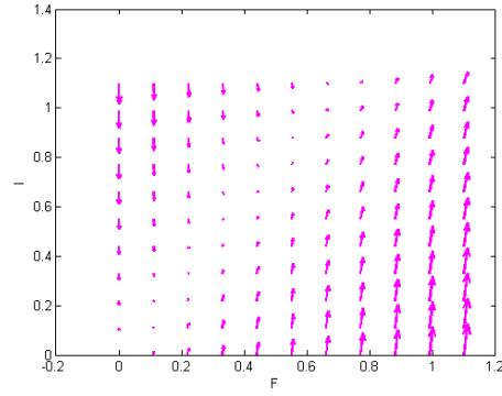
Fig. 9. Behaviour of Foreigner population infected with Covid-19
