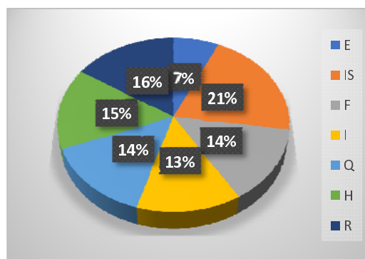
Fig.15. Percentage wise distribution of all the compartments of the model
