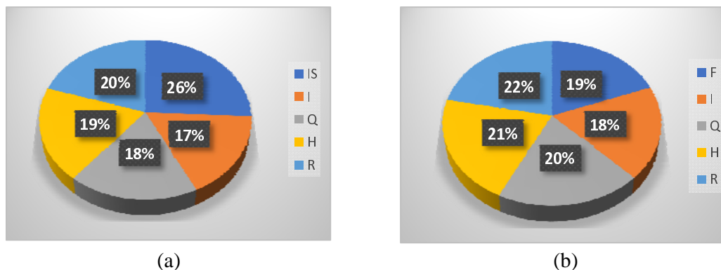
Fig.14. Percentage wise distribution of interstate and foreigner population in Covid-19 scenario
