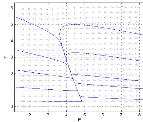
Fig. 5. Phase plot of foreigner when exposed to covid-19
