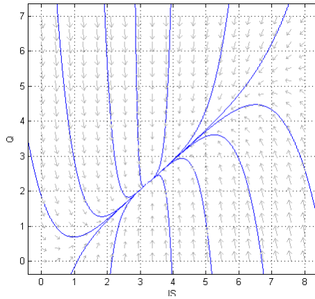
Fig. 6-1. Behaviour of interstate class with quarantine class
