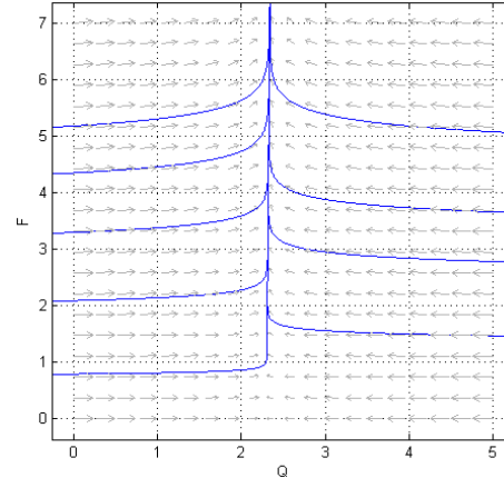
Fig. 6-2. Phase plot of quarantine with foreigners
