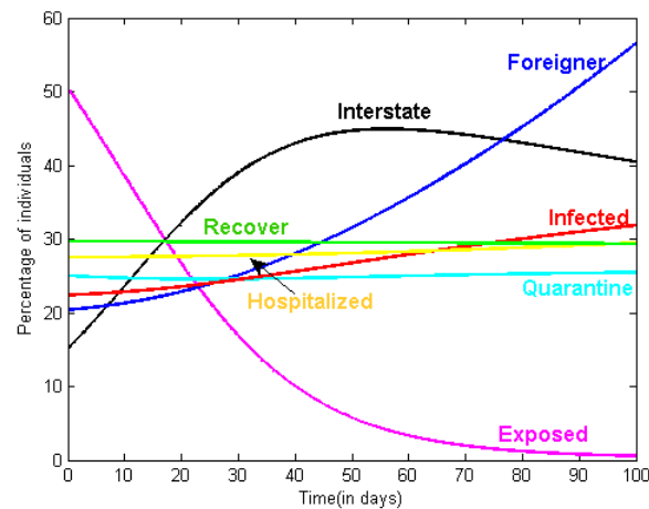
Fig. 2. Transmission of individuals in various compartments
