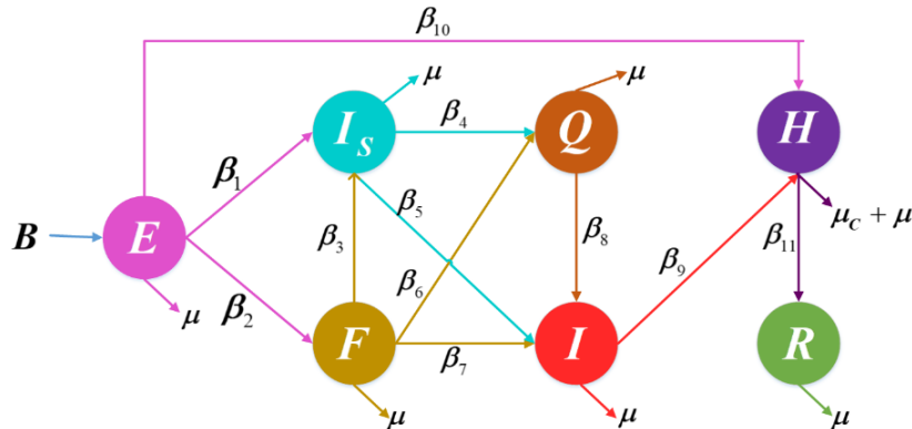
Fig. 1. Movement of individuals from one compartment to another compartment The Fig.1 gives rise to the following set of non-linear ordinary differential equations
