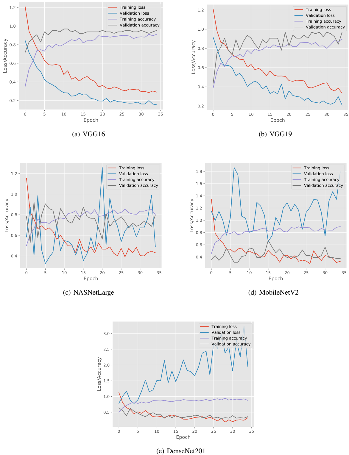
Figure 2: Accuracy and loss (train and test) of deep learning models
