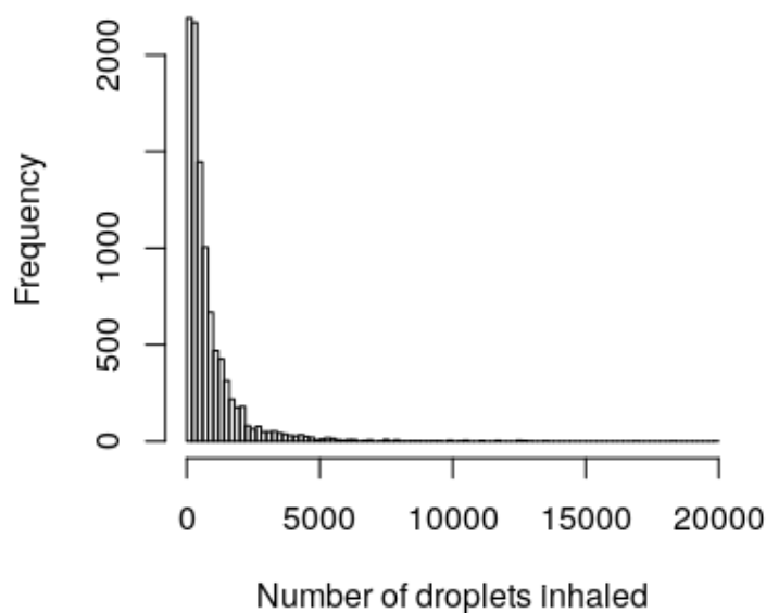
Figure 3. Results of the Scenario 3 'speaking' simulations, showing: (a) the time plot for the median number of particles inhaled and the median particle concentration (x10) in the air; and (b) the distribution of the numbers of particles inhaled, when the ventilation rate is 2 AC/h. Results are for 10,000 simulations.
