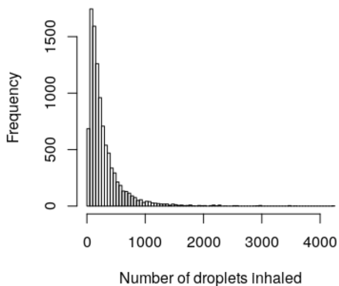
Figure 4. Results of the Scenario 4 'coughing' simulations, showing: (a) the time plot for the median number of particles inhaled and the median particle concentration (x10) in the air; and (b) the distribution of the numbers of particles inhaled, when the ventilation rate is 2 AC/h. Results are for 10,000 simulations.
