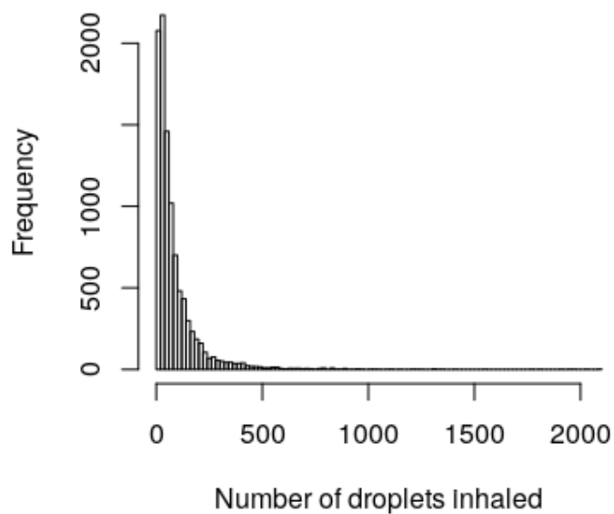
Figure 2. Results of the Scenario 1 'speaking' simulations, showing: (a) the time plot for the median number of particles inhaled and the median particle concentration in the air; and (b) the distribution of the numbers of particles inhaled, when the ventilation rate is 2 AC/h. Results are for 10,000 simulations.
