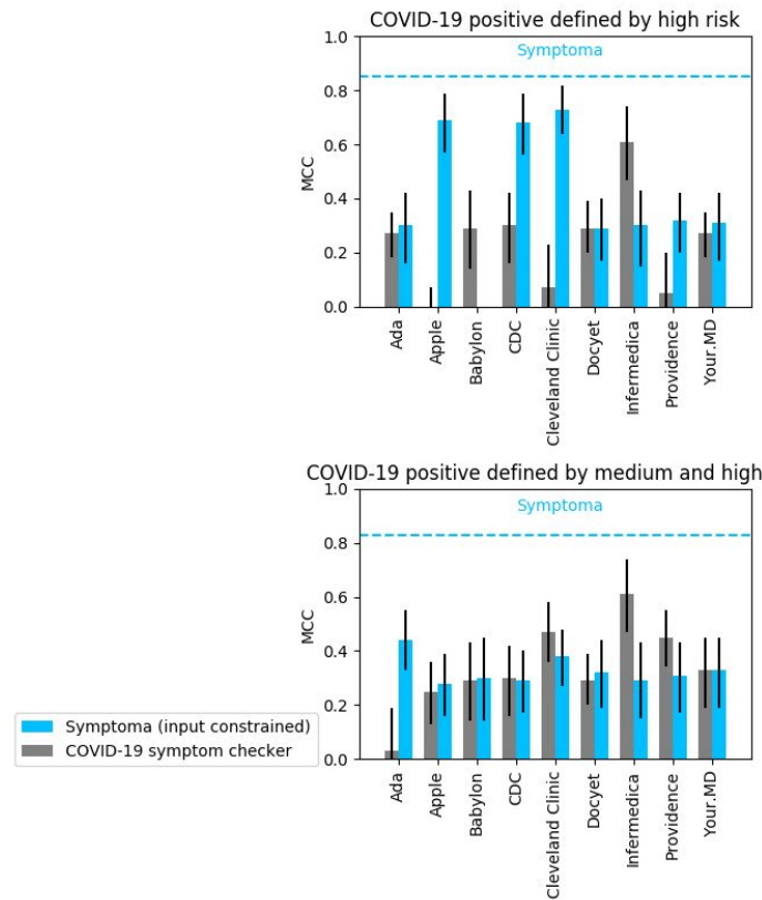
S11 Fig. Pairwise comparison between all symptom checkers and Symptoma based on the MCC if only the subset of symptoms used by one checker is also used for Symptoma.
