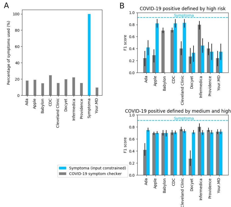
Fig 2. (A) Percentage of symptoms used for case classifications by each symptom checker relative to the total number of symptoms contained in all cases. (B) Symptoma input-constrained evaluation: Pairwise comparison between all symptom checkers and Symptoma based on the F1 score if only the subset of symptoms used by one checker is also used for Symptoma. The same analysis based on the MCC is shown in the S11 Fig . Please note that using only Babylon's symptom inputs all cases are either classified medium or low risk by Symptoma and therefore there is no bar in the upper panel for Babylon's Symptoma.
