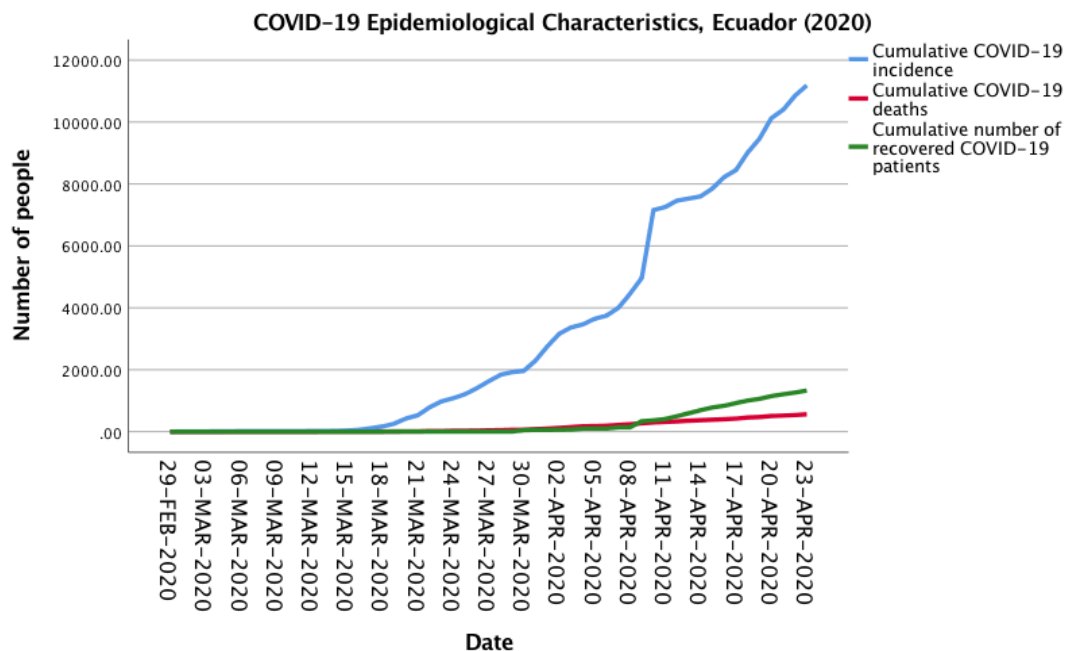
Figure 2. Epidemiological characteristics of the COVID-19 outbreak in Ecuador
