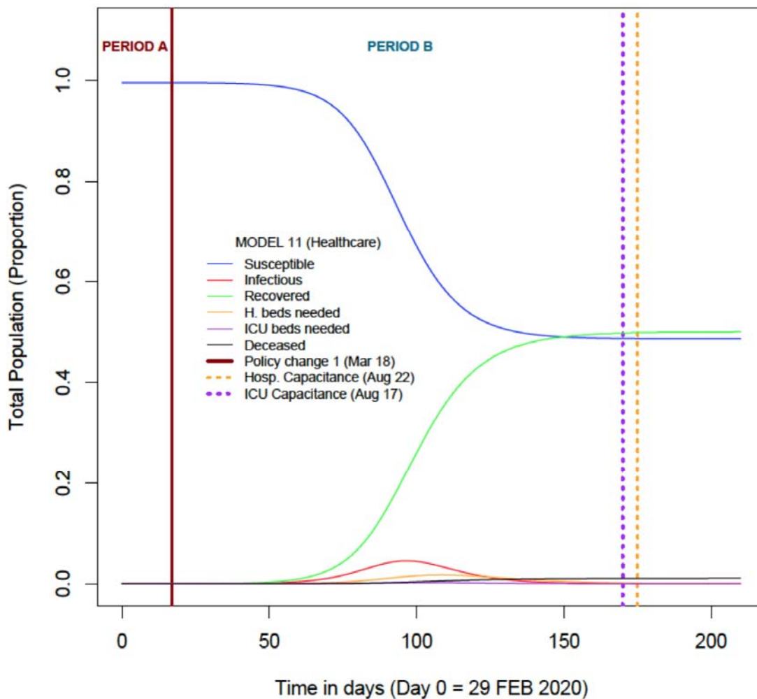
Figure 4A. MODEL 11: HeCEM-simulated COVID-19 outbreak in Ecuador. Solid line represents the time when containment measures were enacted. Dashed lines represent time at which capacitance is reached.
