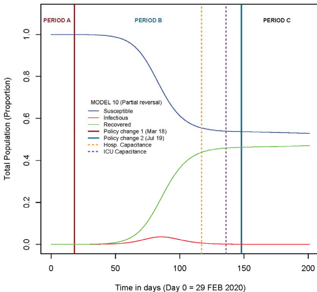
Figure 3C. MODEL 10: SIR-simulated COVID-19 outbreak in Ecuador if containment measures are partially reversed on July 19 th , 2020. Solid lines represent period boundaries. Dashed lines represent time at which capacitance is reached.
