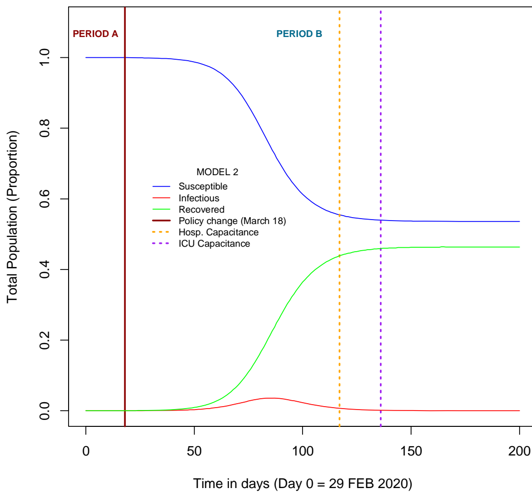
Figure 3B. MODEL 2: SIR-simulated COVID-19 outbreak in Ecuador, accounting for the start of containment measures.
