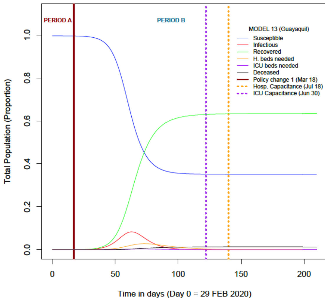
Figure 4C. MODEL 13: HeCEM-simulated COVID-19 outbreak in Guayaquil. Solid lines represent time when COVID-19 policies change. Dashed lines represent time at which capacitance is reached.
