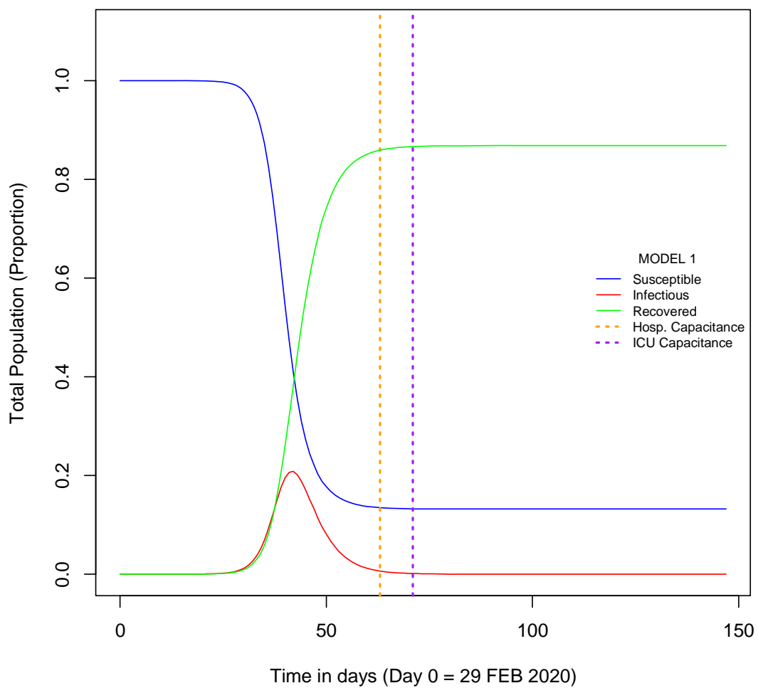
Figure 3A. MODEL 1: Ecuador COVID-19 initial SIR Model.
