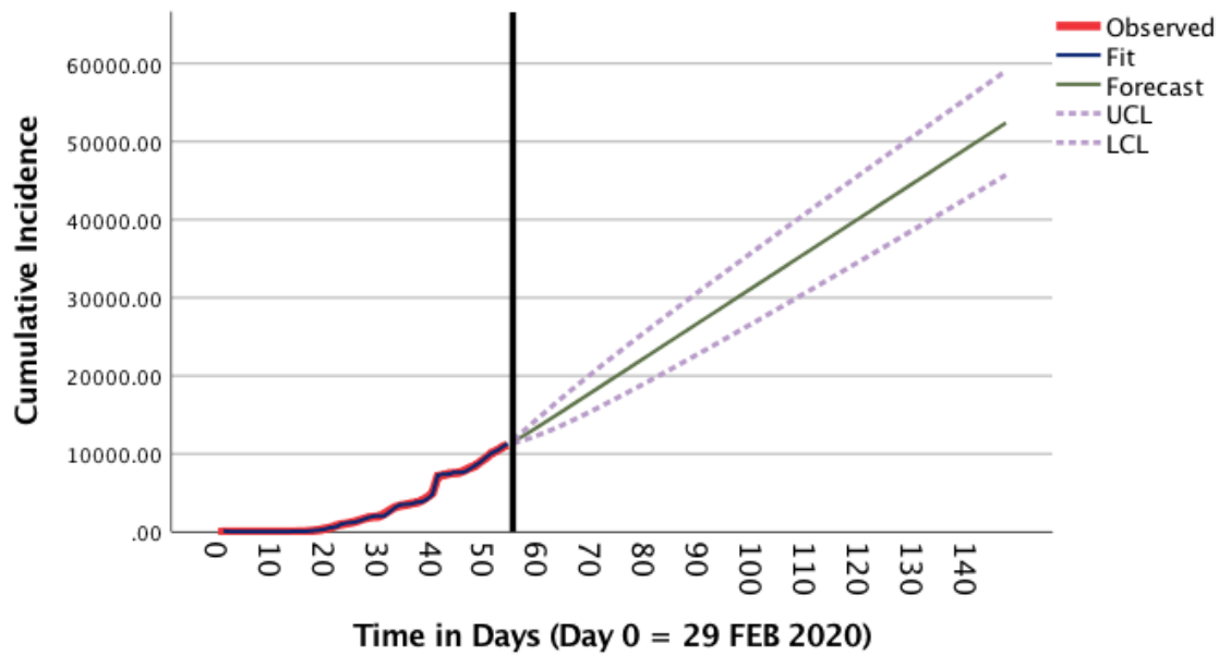
Figure 5. Forecast of COVID-19 cumulative reported incidence.
