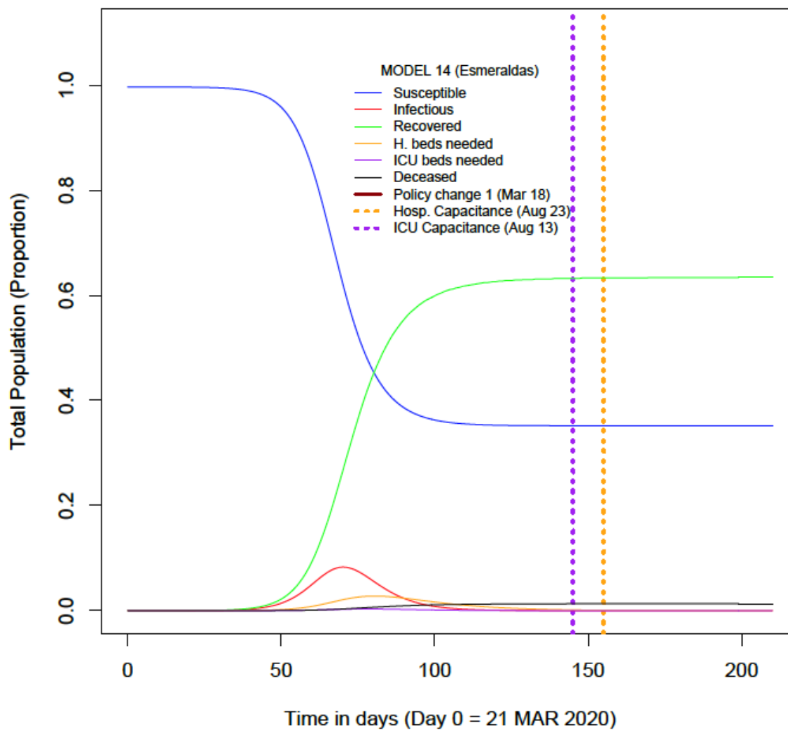
Figure 4D. MODEL 14: HeCEM-simulated COVID-19 outbreak in Esmeraldas. Dashed lines represent time at which capacitance is reached.
