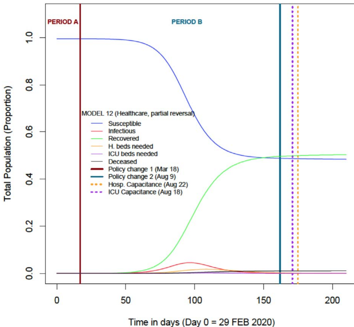
Figure 4B. MODEL 12: HeCEM-simulated COVID-19 outbreak in Ecuador assuming a partial reversal of containment measures on August 9 th . Solid lines represent time when COVID-19 policies change. Dashed lines represent time at which capacitance is reached.
