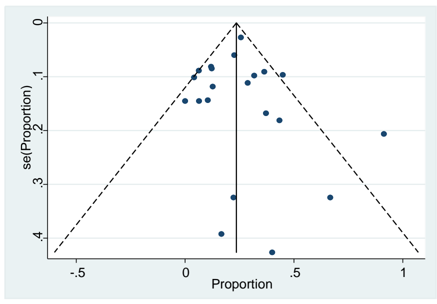
Figure 5. Funnel Plot for Meta-Analysis of COVID-19 Asymptomatic Proportion in Community Studies
